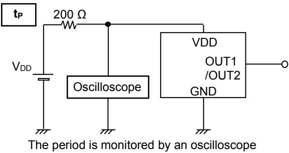
Figure 2. t P Measurement Circuit
