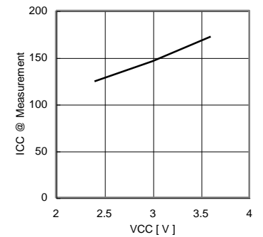
Fig.9 VCC - ICC (During measurement)
