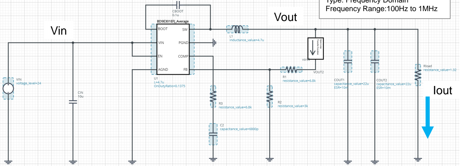
Figure 1. Simulation Schematic
