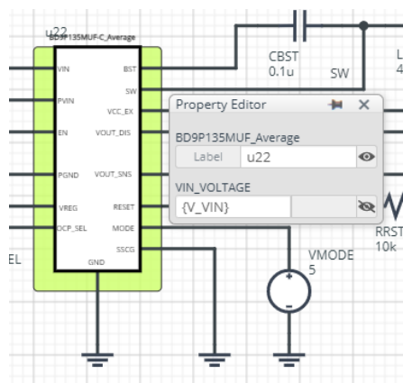
Figure 4. Property Editor of BD9P135MUF-C_Average model
