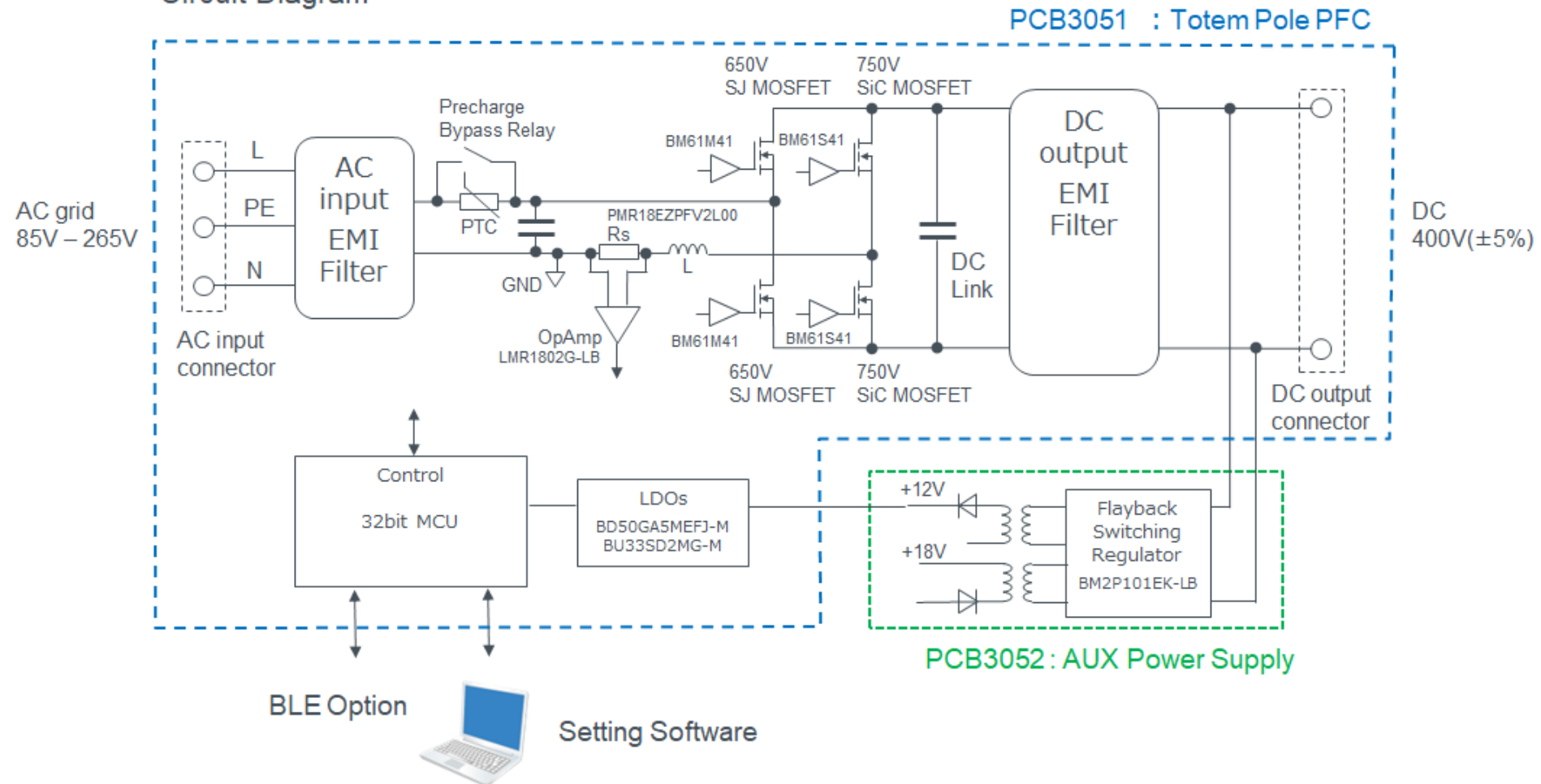
APEVK66001 3.6kW Totem Pole PFC with 4 th Gen. SiC MOSFET Circuit Diagram
