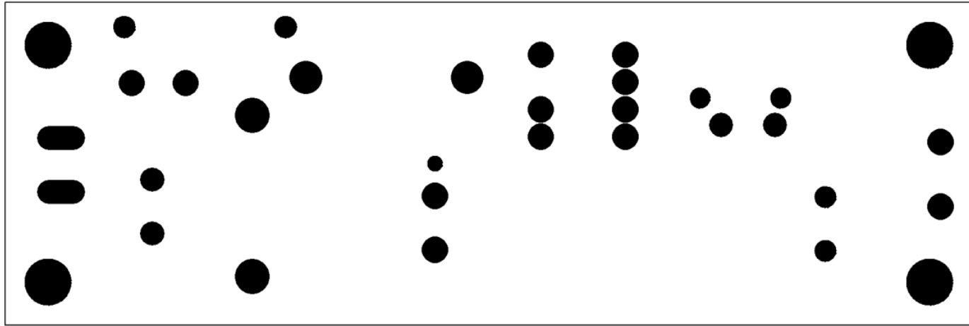
TOP_Mask
