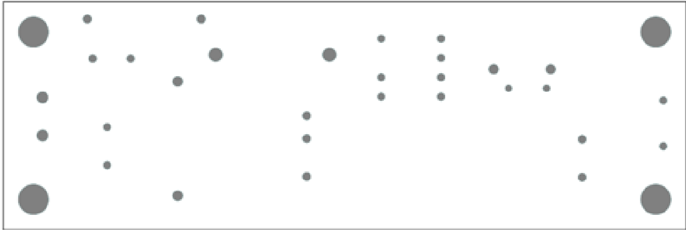
Drill
