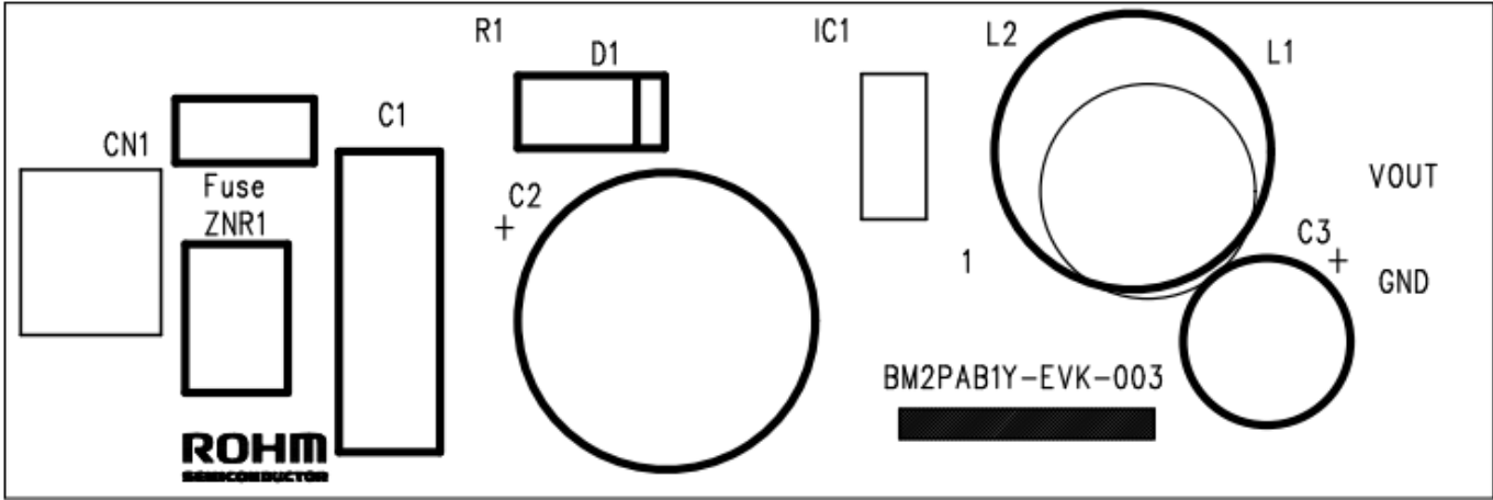
Top_Silk
