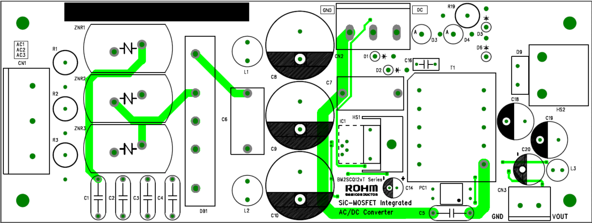
Top Layout(Top view)
