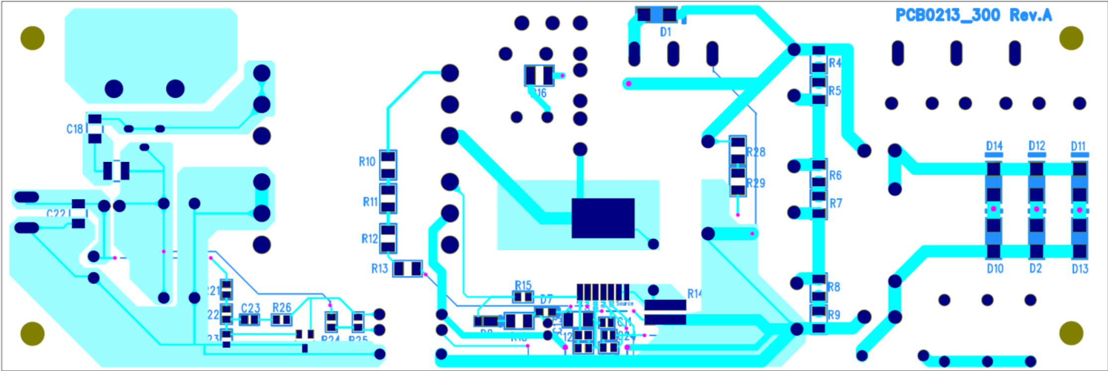
Bottom view
