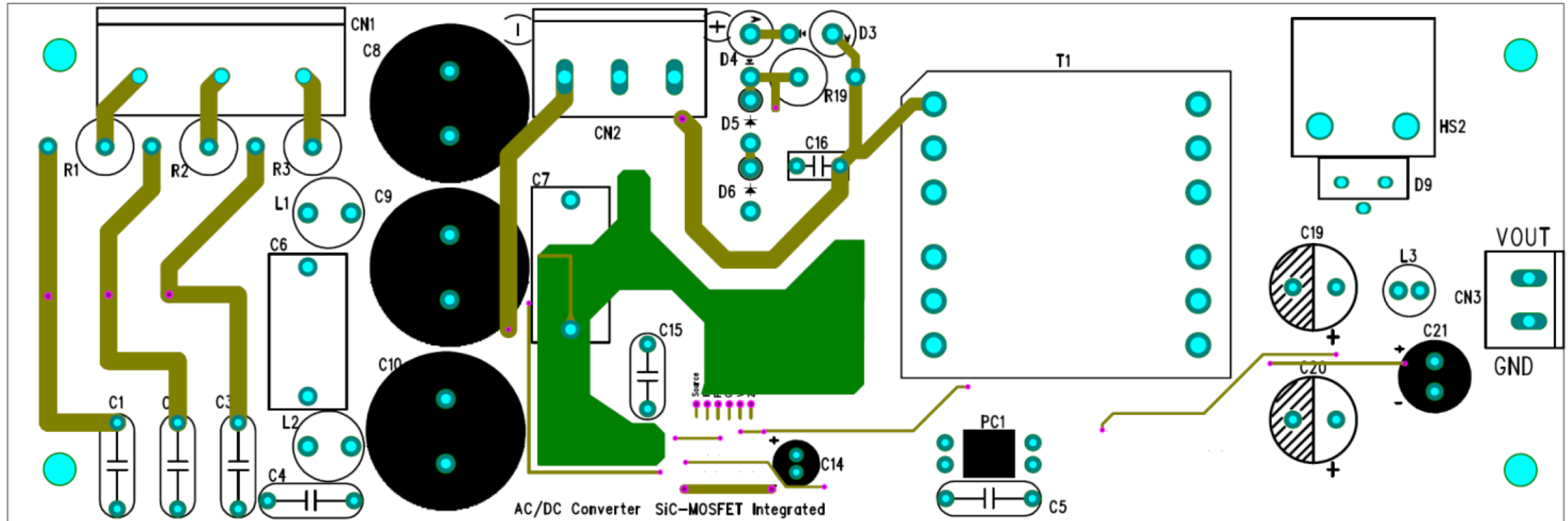
Top view
