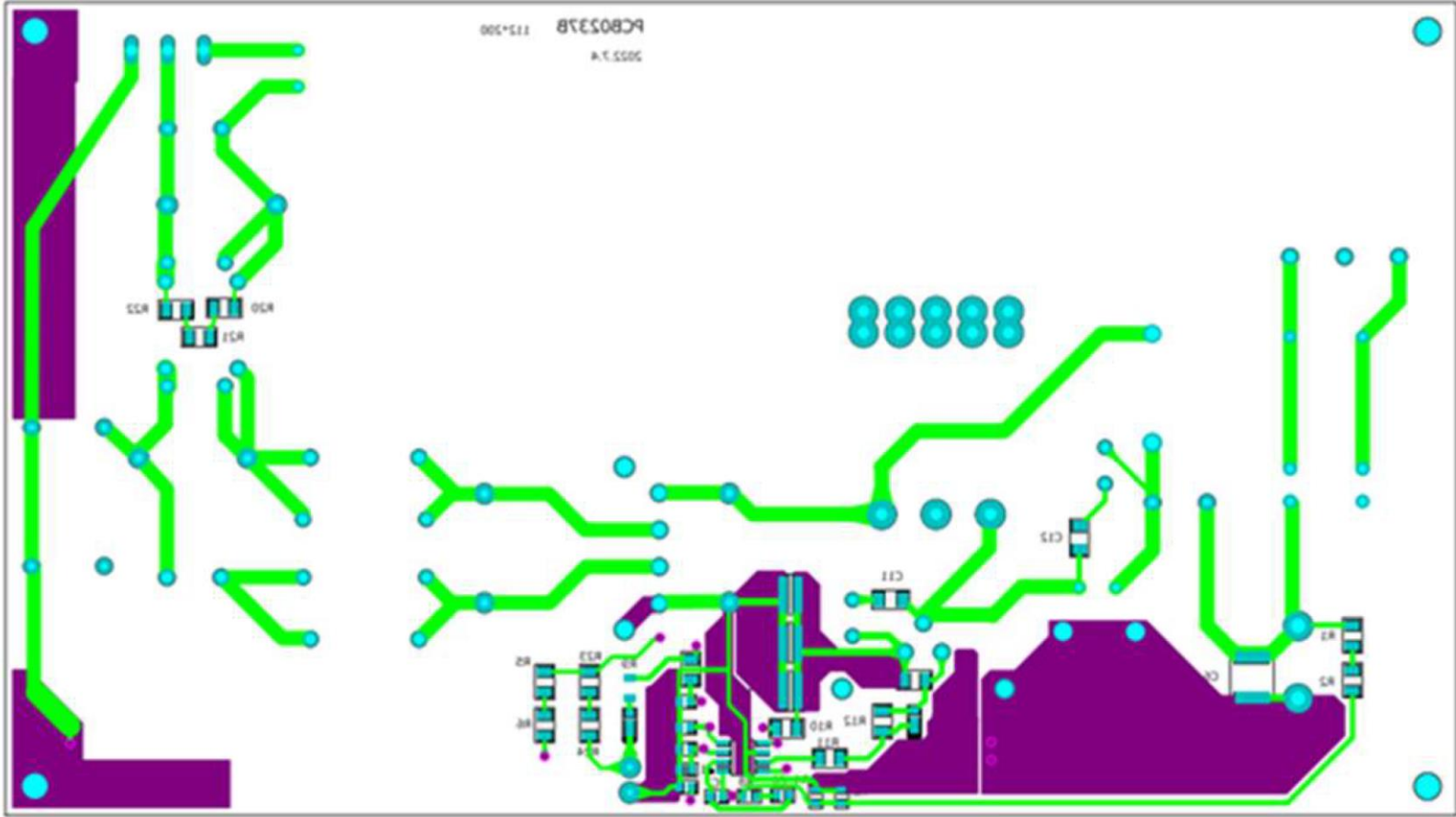
Bottom Layout
