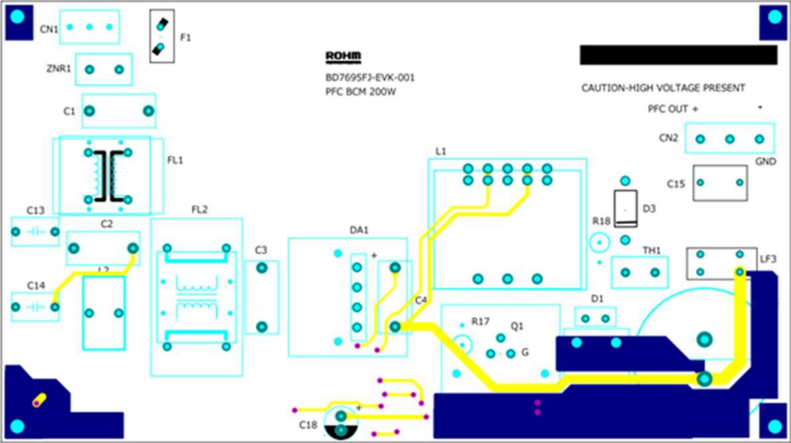
Top Silkscreen
