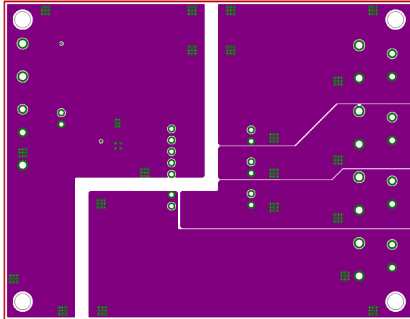
Middle Layer2 Layout
