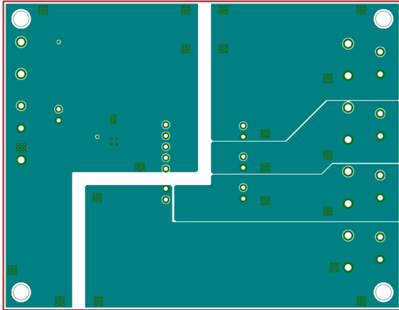
Middle Layer1 Layout
