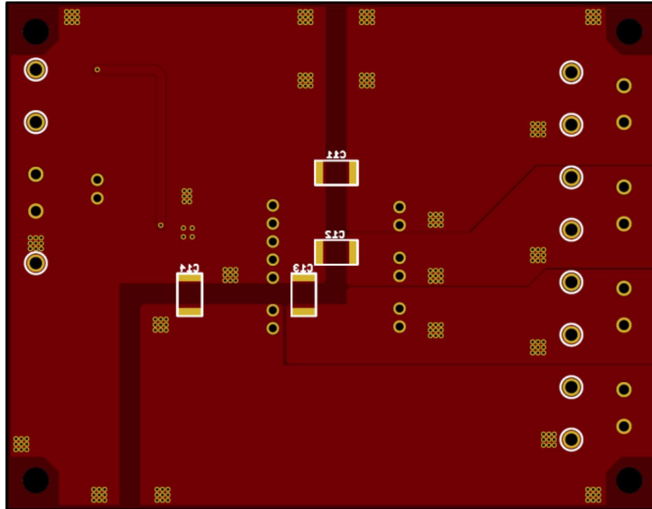
Bottom Silk Screen and Layout
