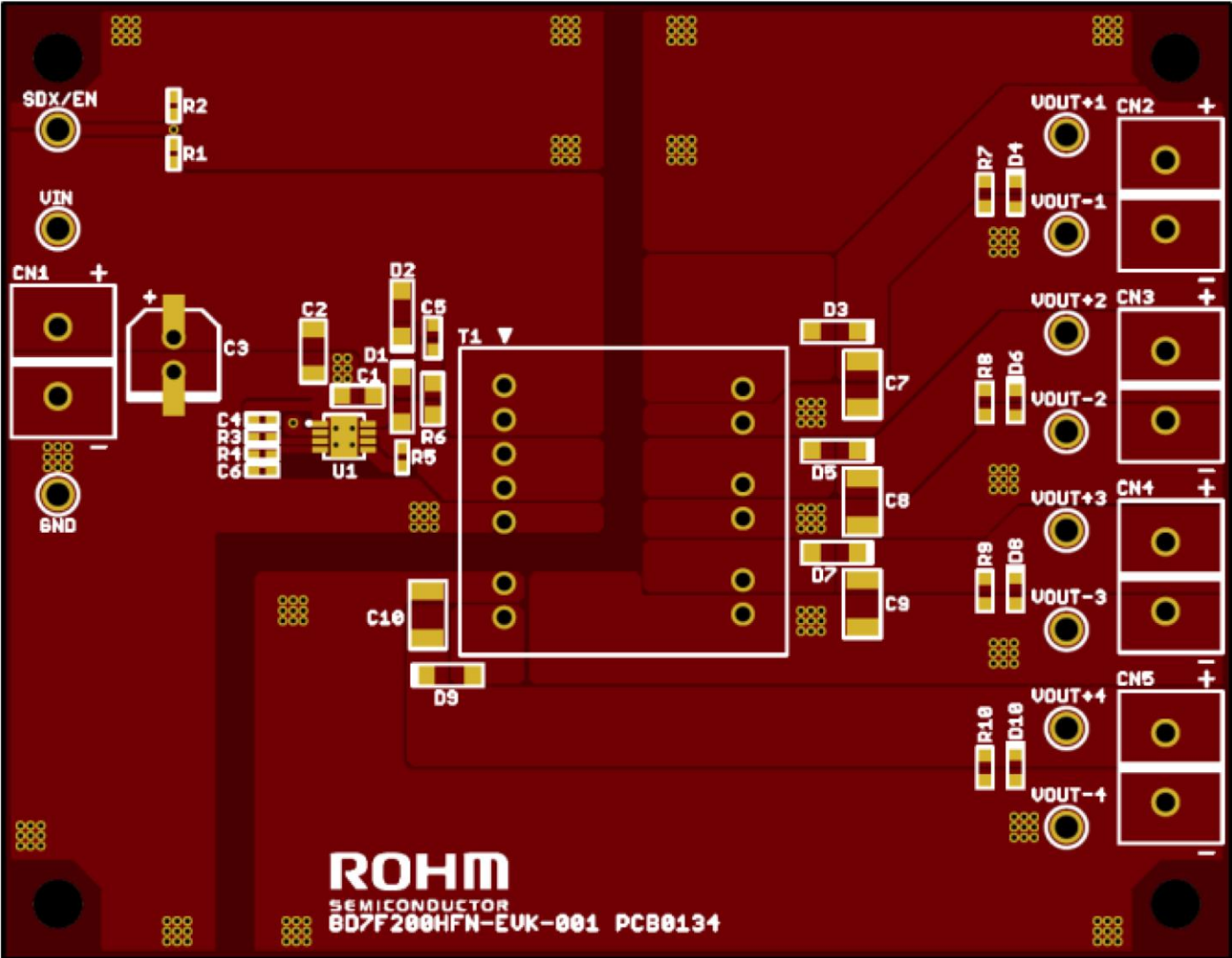
Top Silk Screen and Layout
