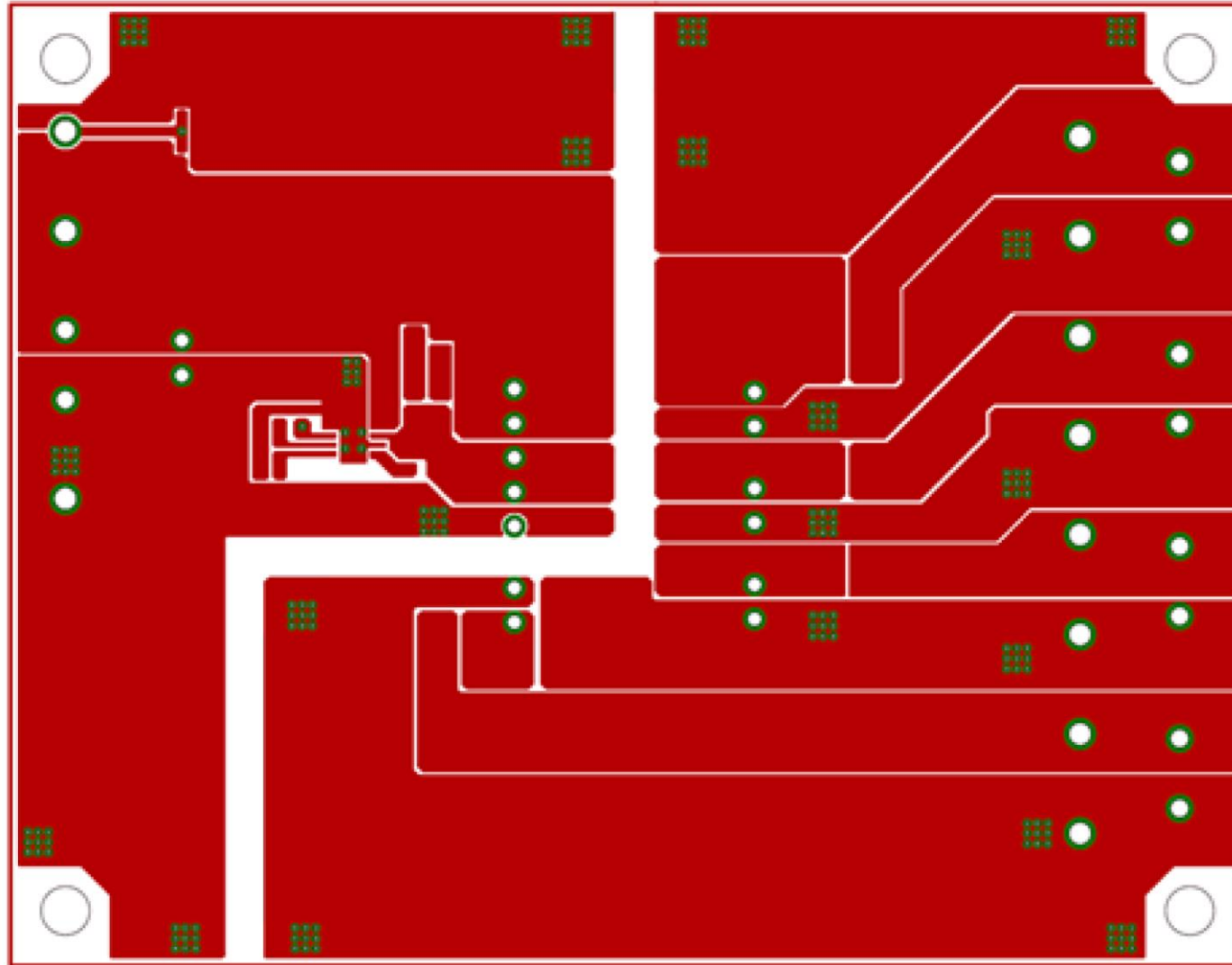
Top Side Layout
