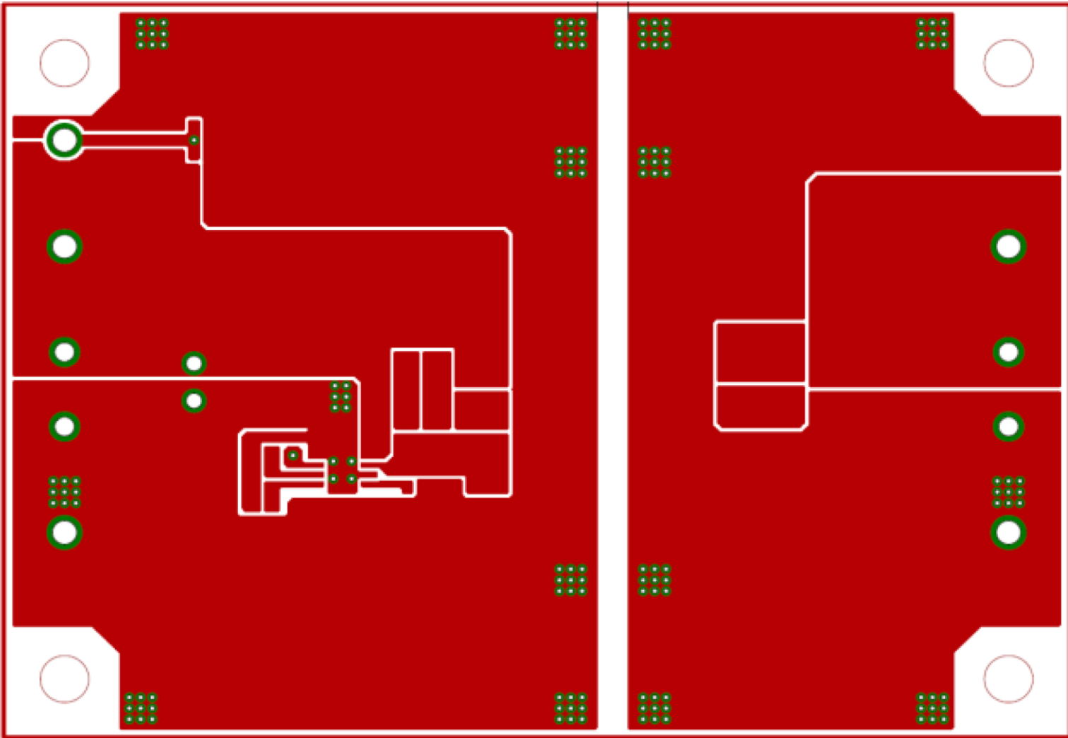
Top Side Layout
