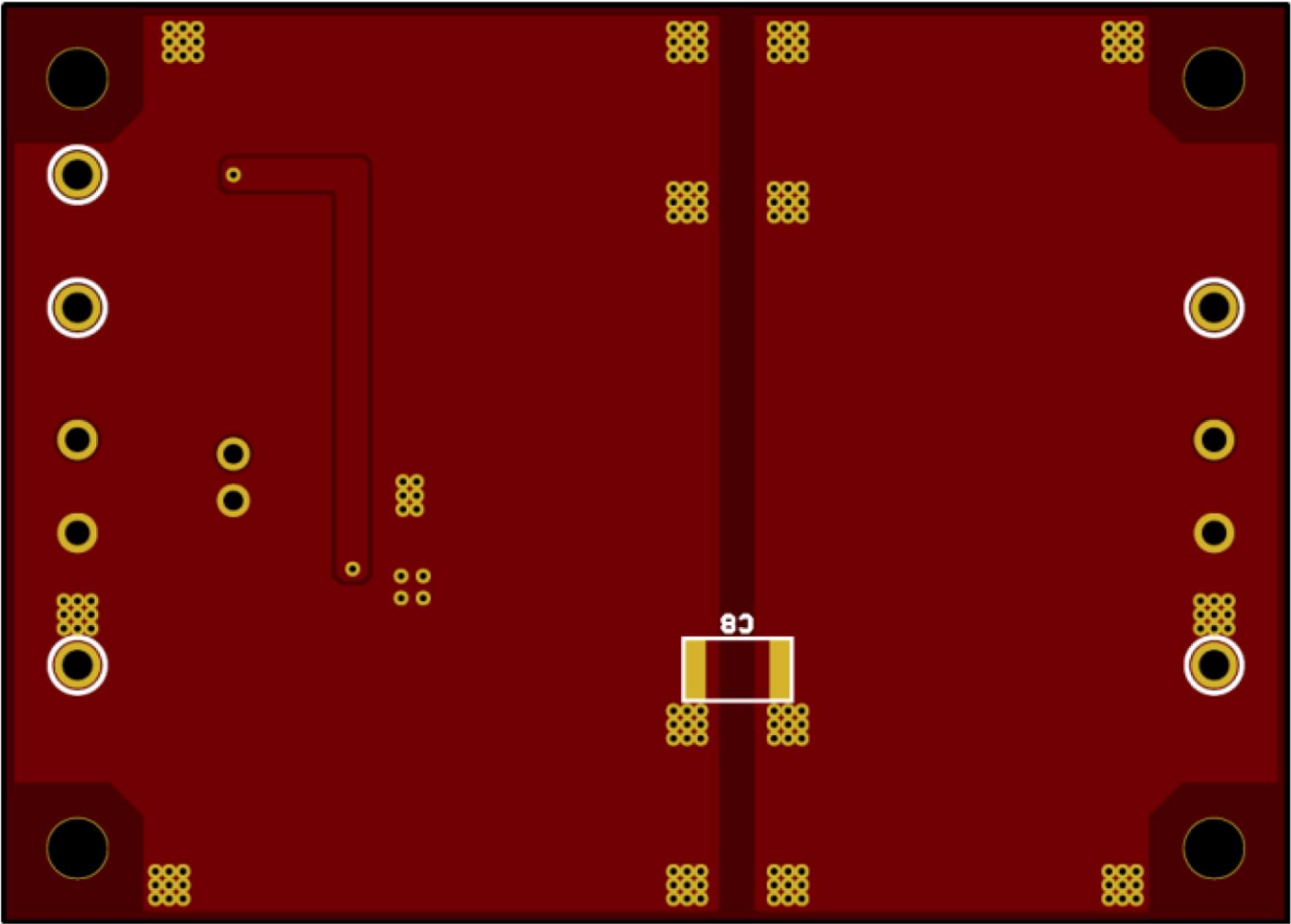
Bottom Silk Screen and Layout
