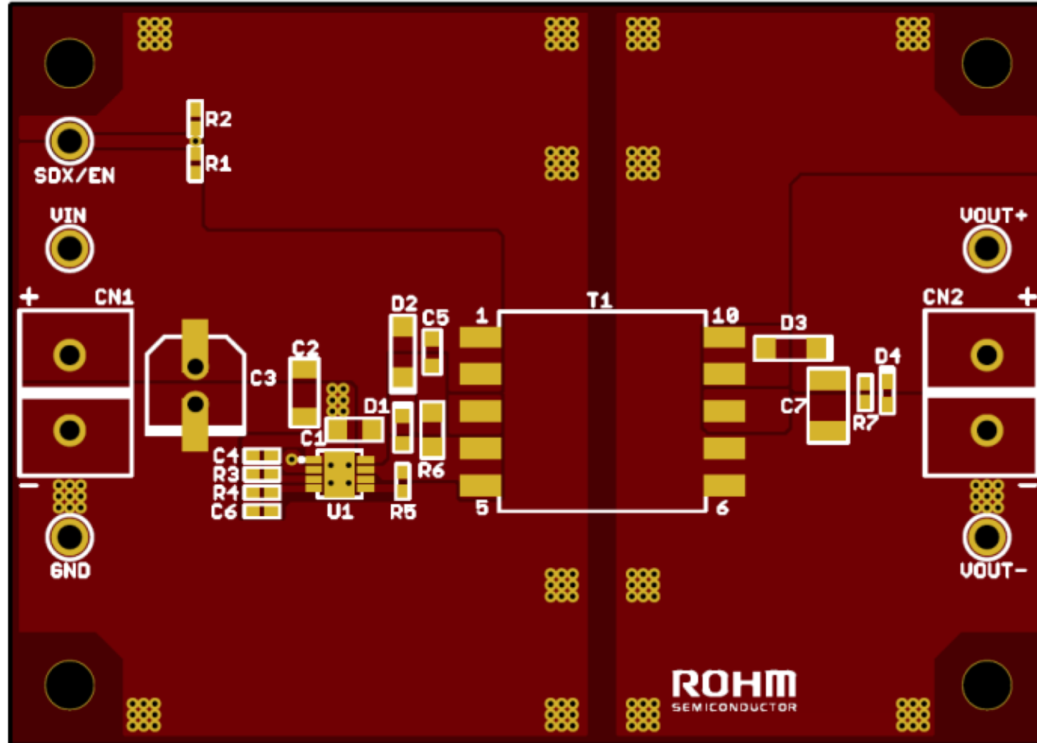
Top Silk Screen and Layout
