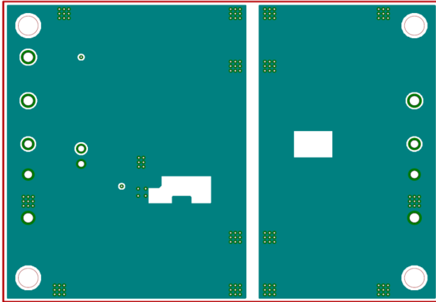
Middle Layer1 Layout
