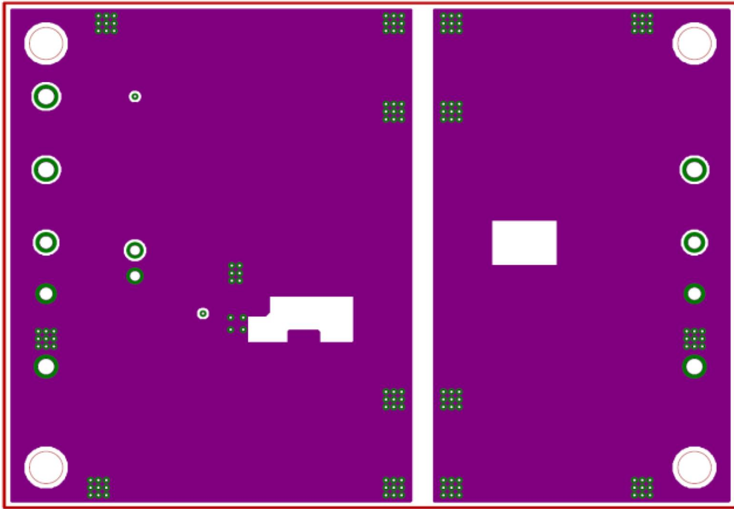
Middle Layer2 Layout
