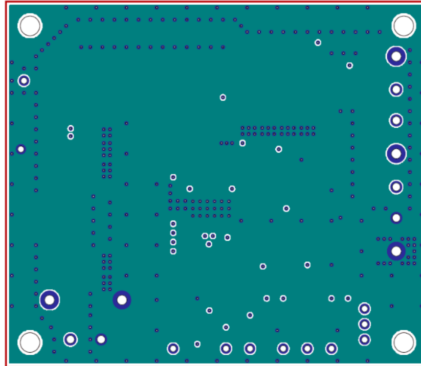
2nd layer layout(Top view)
