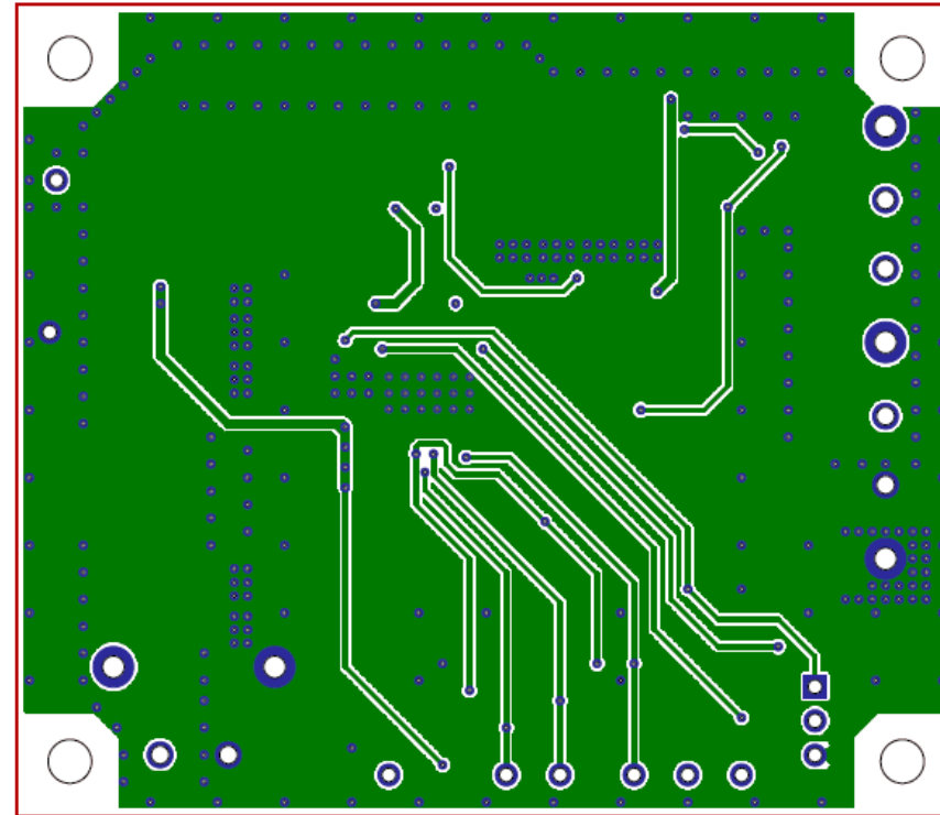
Bottom layer layout(Top view)
