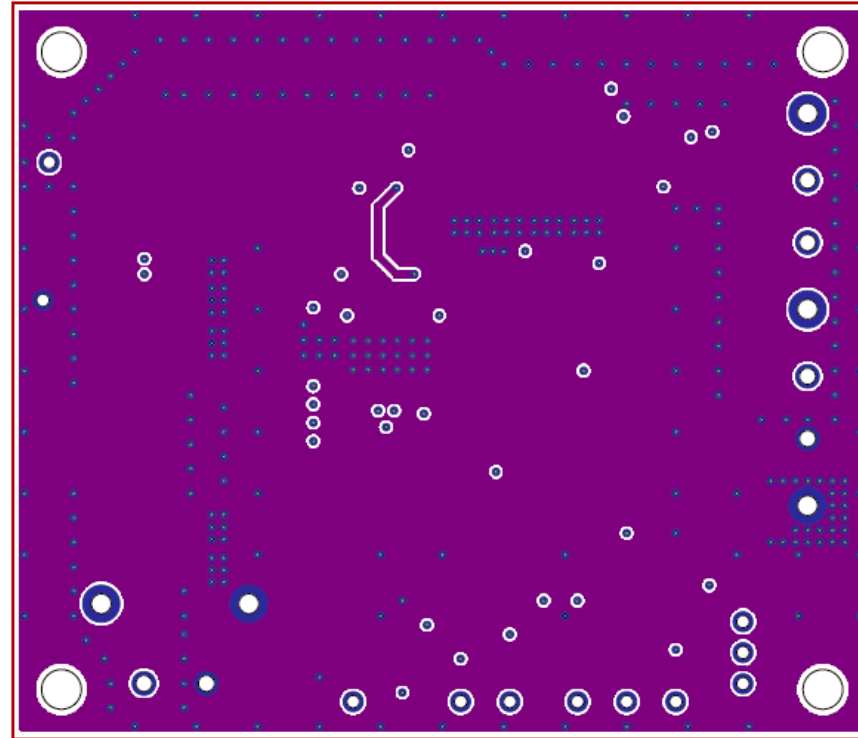
3rd layer layout(Top view)
