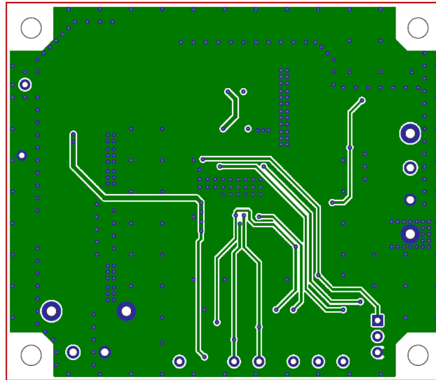
Bottom layer layout(Top view)
