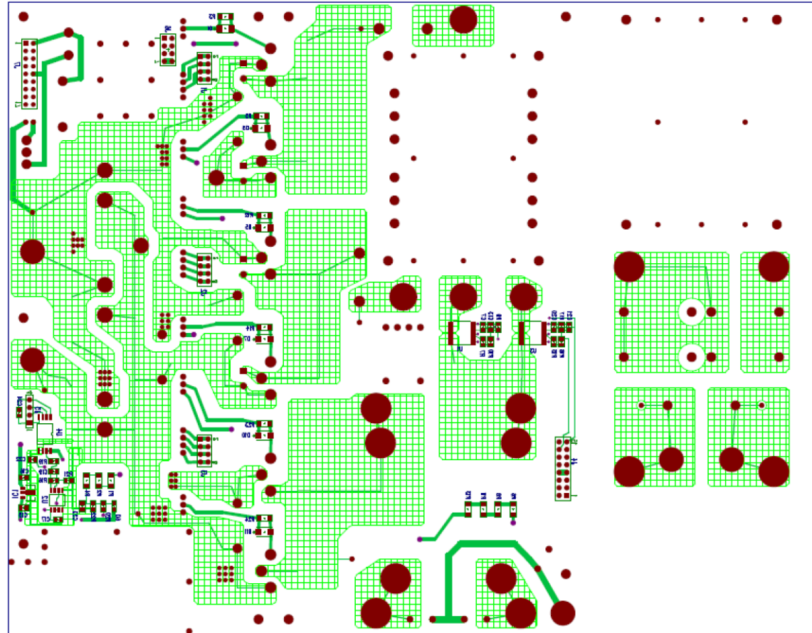
Bottom View
