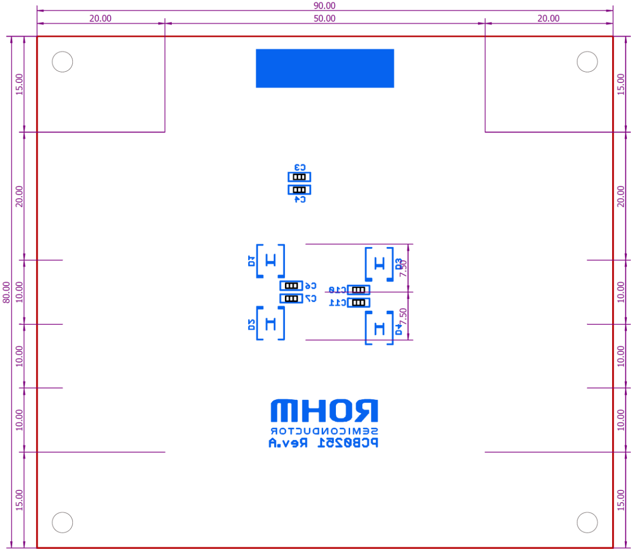
Top View Bottom Silkscreen Overlay
