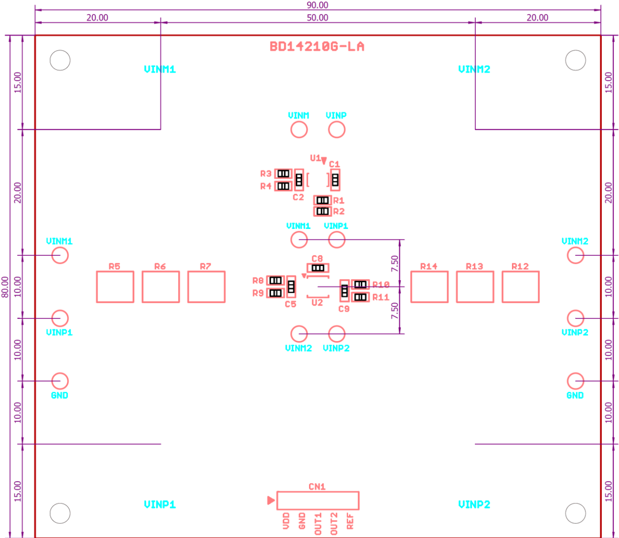
Top View Top Silkscreen Overlay
