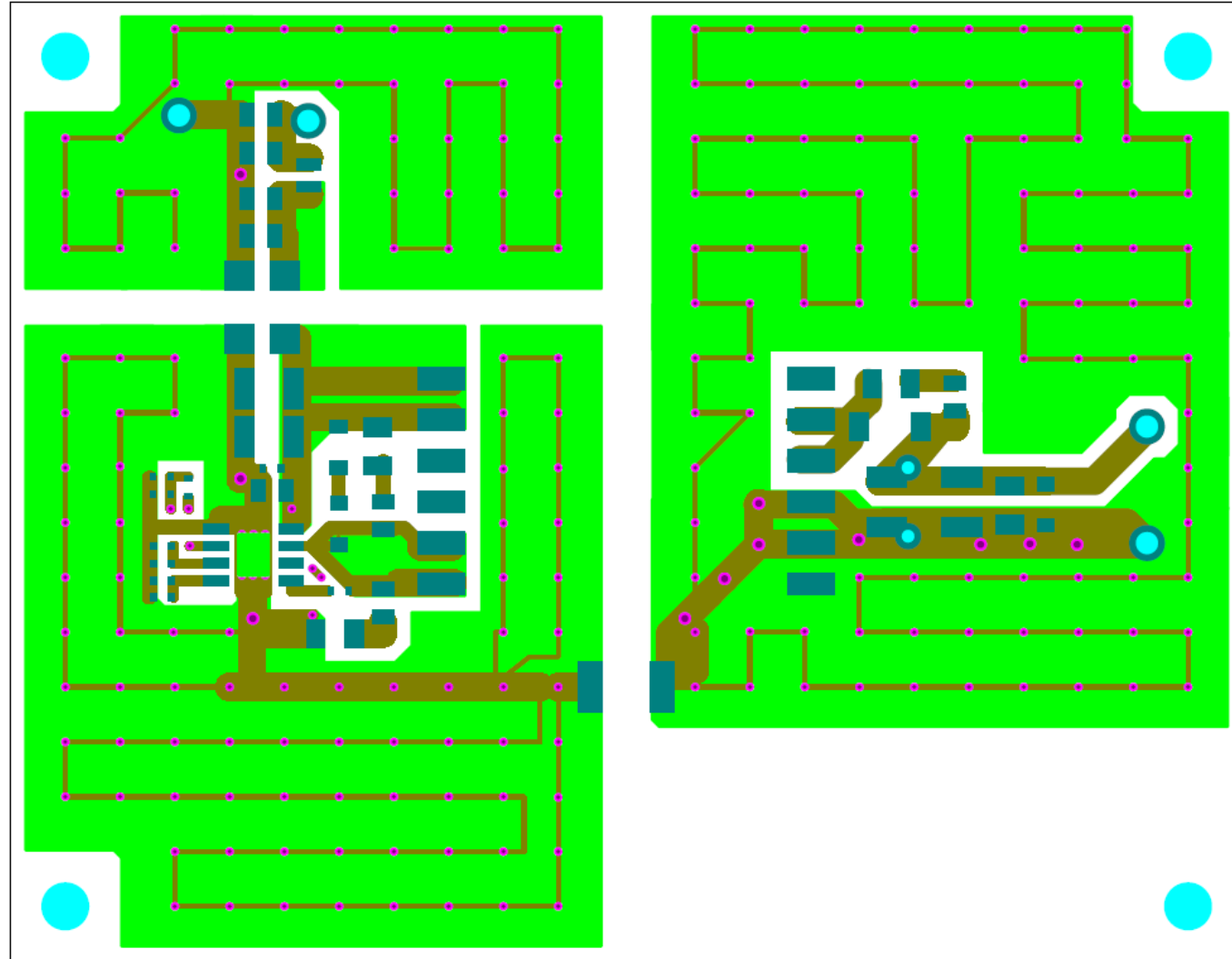
Top Pattern layout (Top View)
