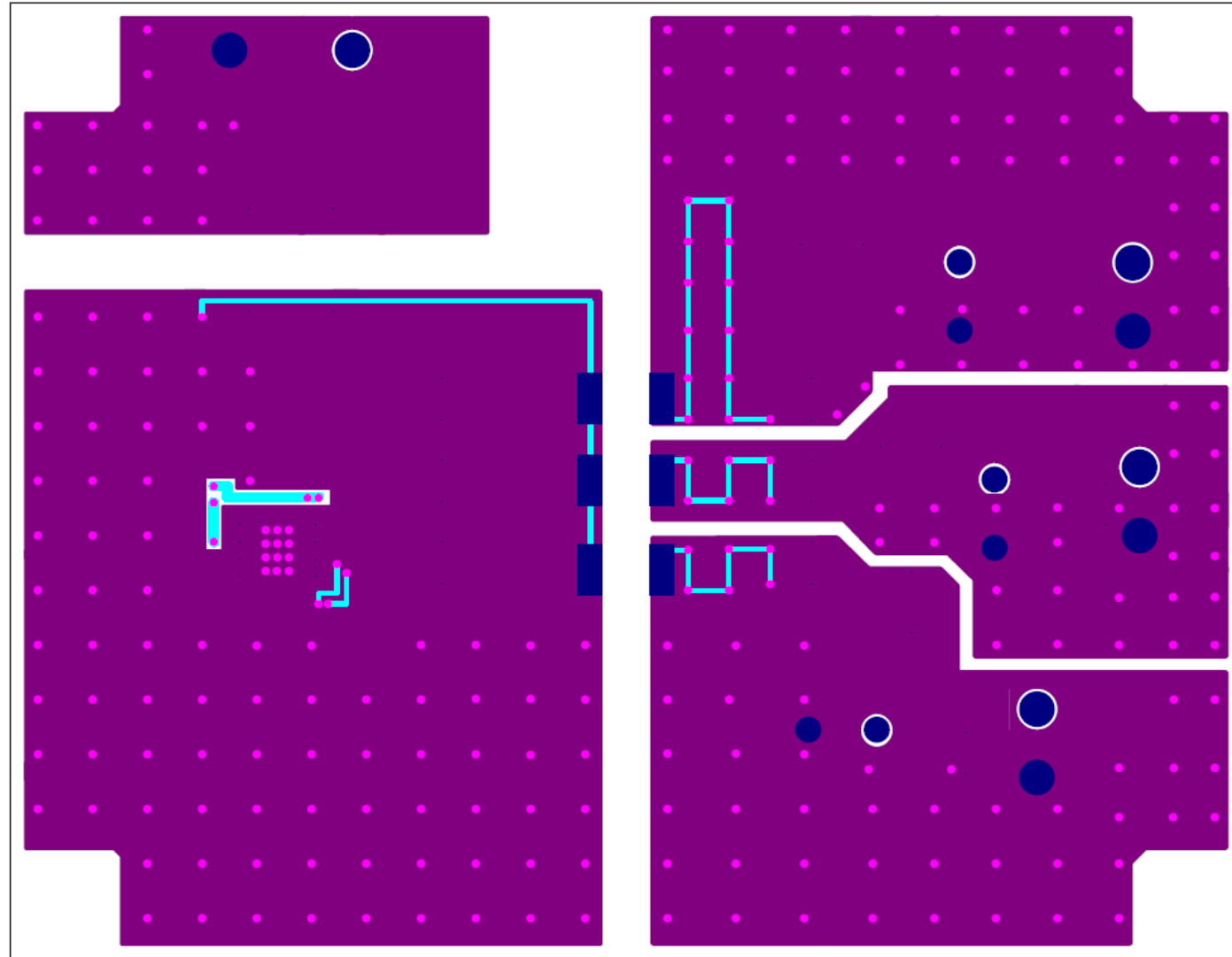
Bottom Pattern layout (Top View)
