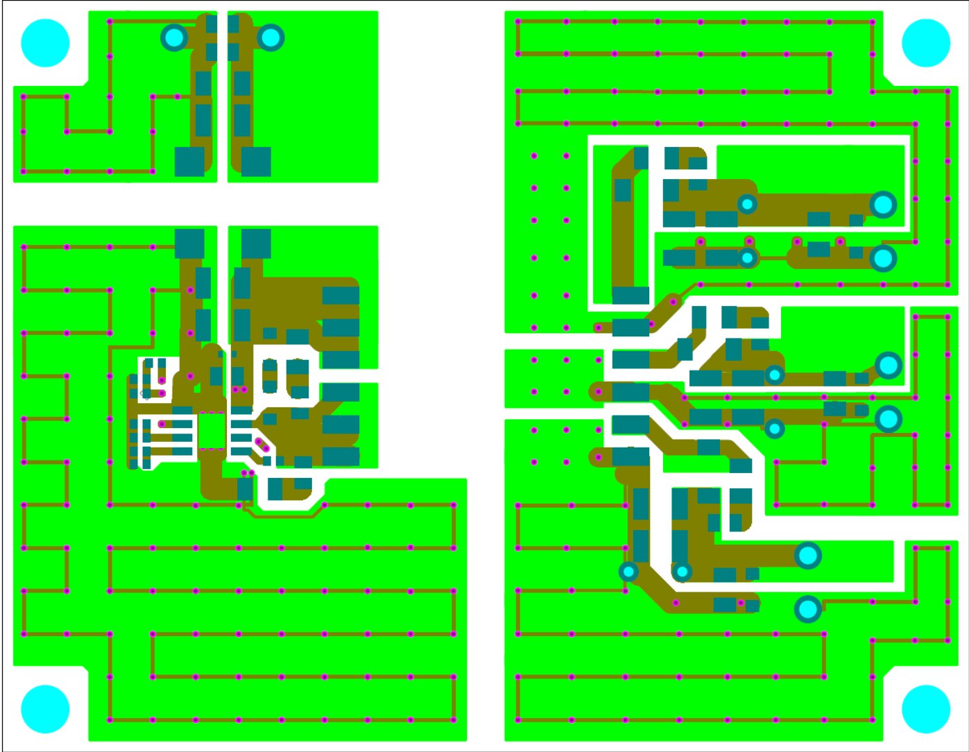
Top Pattern layout (Top View)
