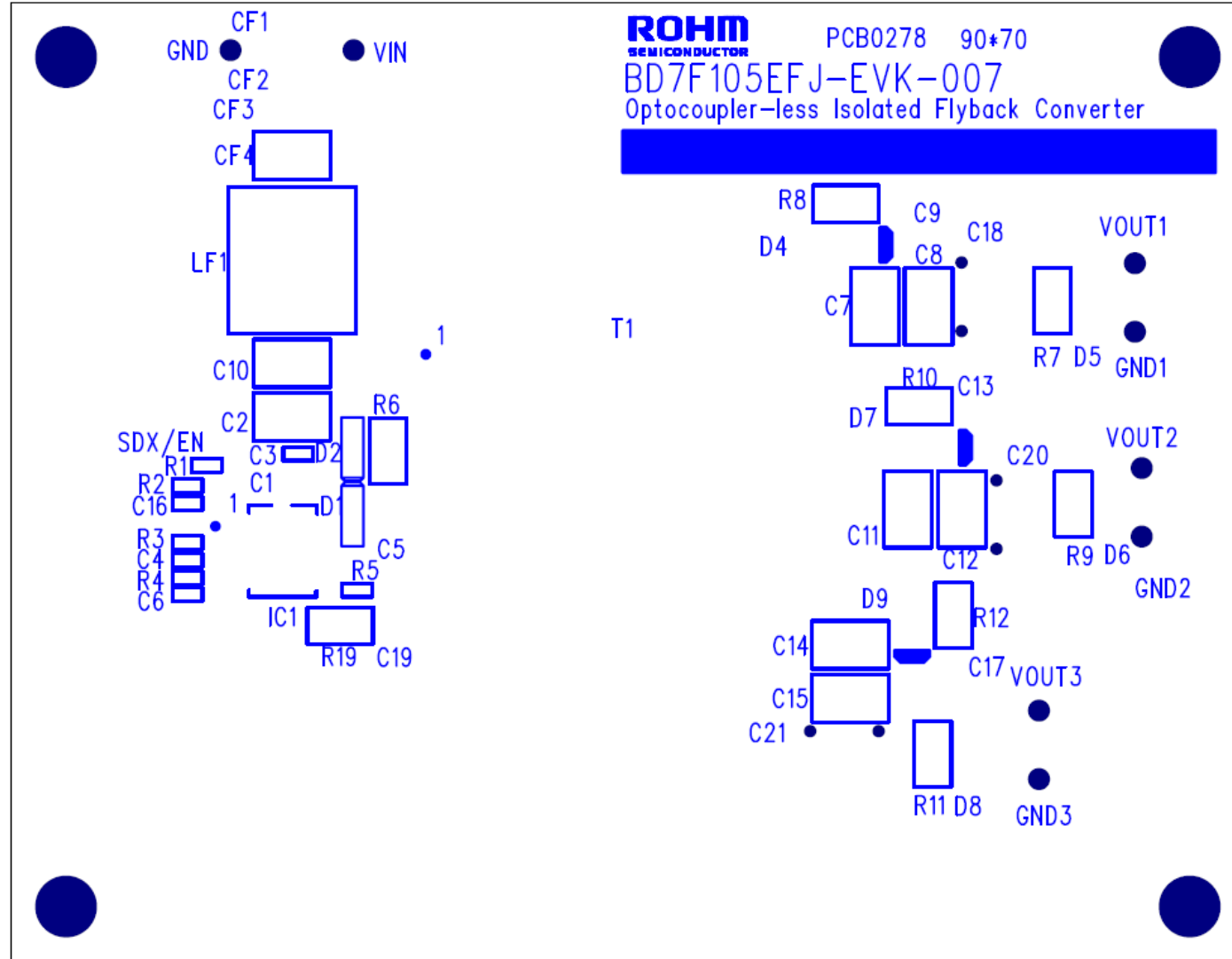
Top Silk layout (Top View)
