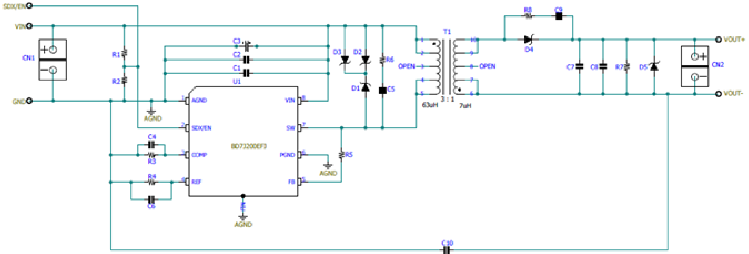
BD7J200EFJ-EVK-001 Circuit Diagram
