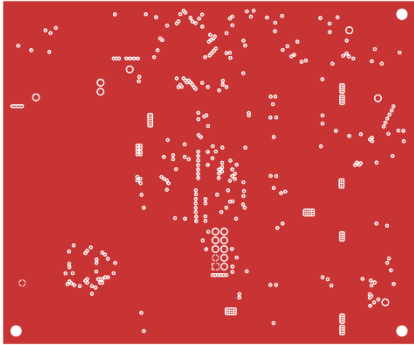
Figure 7. Mid1 layer layout (Top view)
