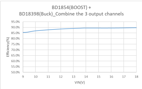
Figure 13. Efficiency
