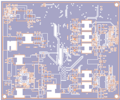
Figure 6. Top layer layout (Top view)
