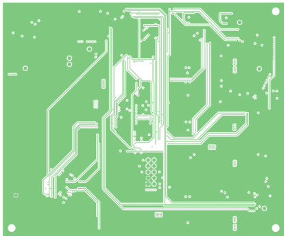
Figure 8. Mid2 layer layout (Top view)
