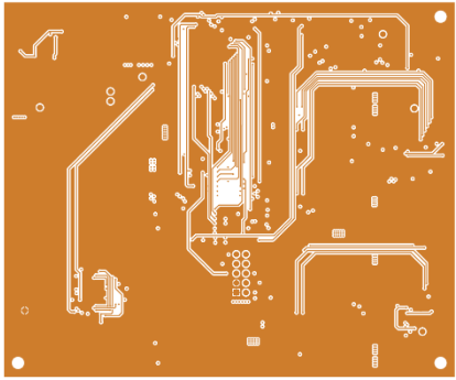
Figure 9. Mid3 layer layout (Top view)
