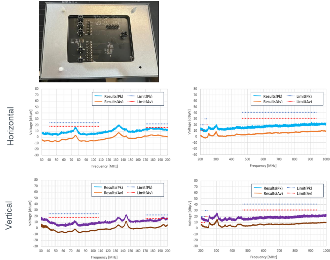
Figure 12. Radiated noise (CISPR25 Class5)
