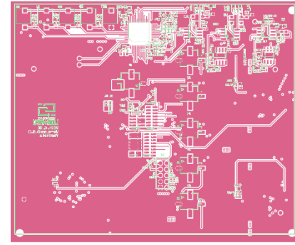
Figure 11. Bottom layer layout (Top view)
