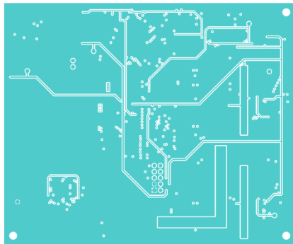
Figure 10. Mid4 layer layout (Top view)
