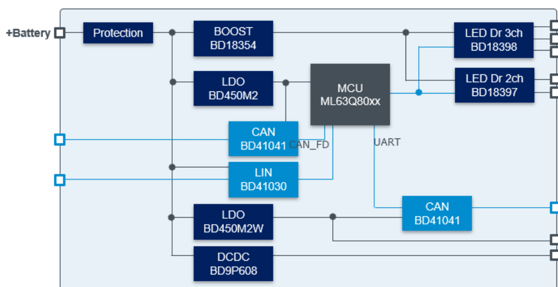
Figure1: Block diagram
