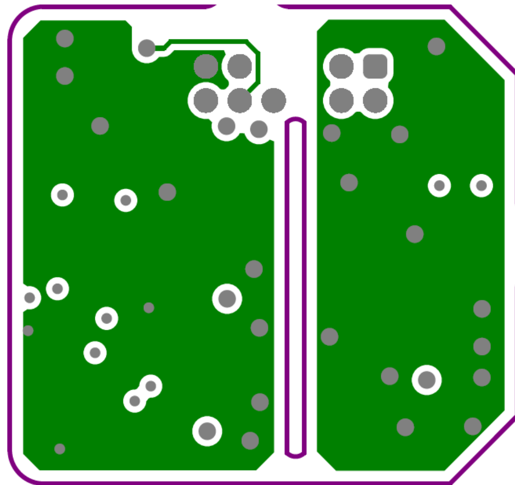
[Mid layer 1] (Top View)
