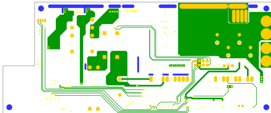
• 3rd layer
