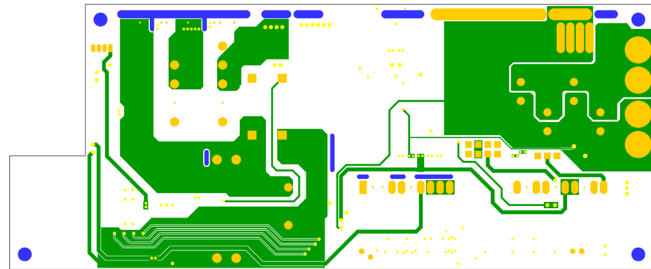
• 2nd layer
