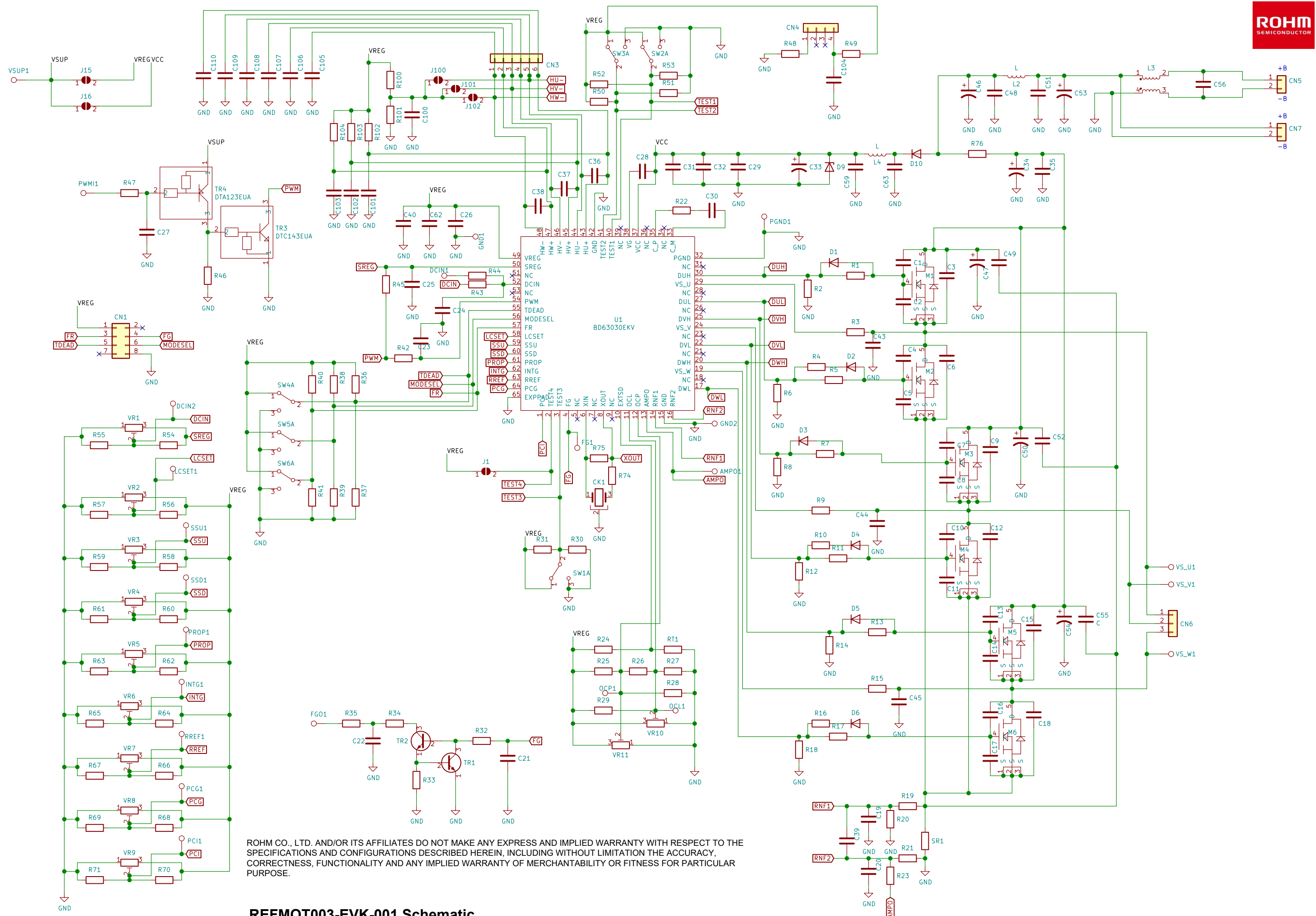
REFMOT003-EVK-001 Schematic
