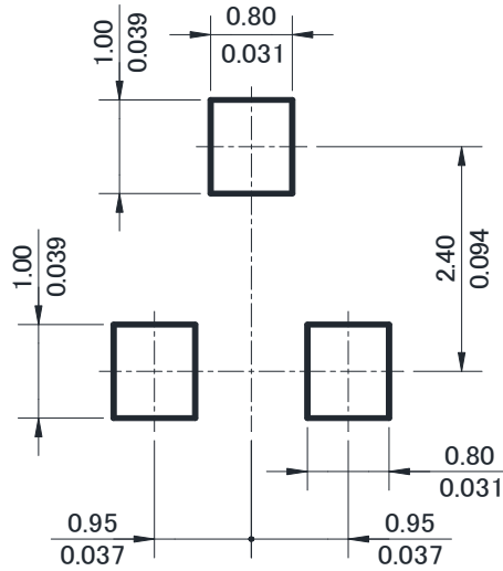
Soldering footprint
