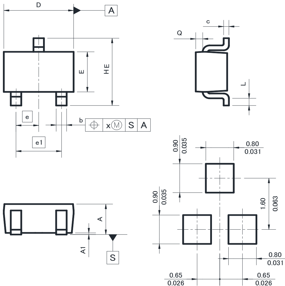
Soldering footprint
