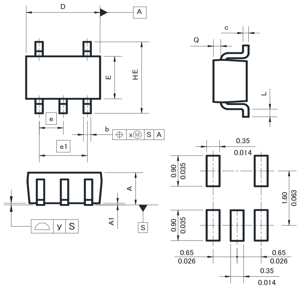
Soldering footprint
