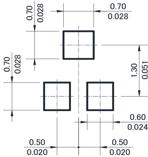
Soldering footprint
