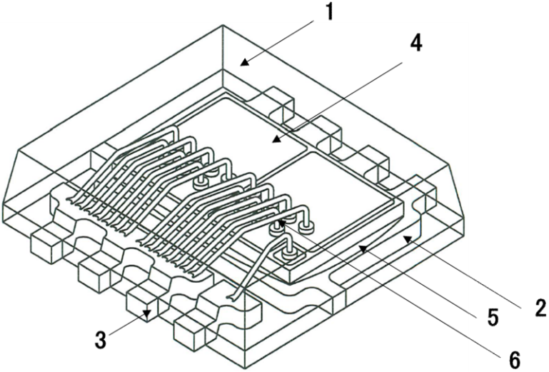
A direction of wire bonding and die bonding, a shape of frame, die size and the number of wires differ by P/N.
