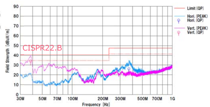
Figure 24. Radiated Emission.2 V IN =230Vac/50Hz, I OUT =0.5A QP margin= 6.4dB, AV margin=8.4dB
