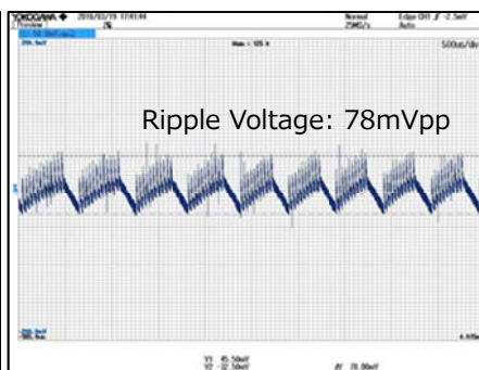
Figure 19. VOUT Ripple Voltage.5 V_{IN}=230Vac , I_{OUT}=100mA CH1: VOUT 50mV/div, 500µs/div
