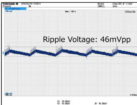
Figure 15. VOUT Ripple Voltage.1 V_{IN}=100Vac , I_{OUT}=10mA CH1: VOUT 50mV/div, 500µs/div
