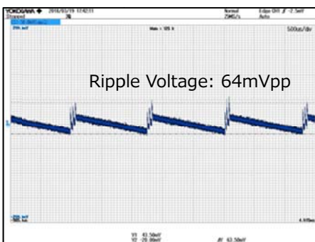
Figure 18. VOUT Ripple Voltage.4 V_{IN}=230Vac , I_{OUT}=10mA CH1: VOUT 50mV/div, 500µs/div
