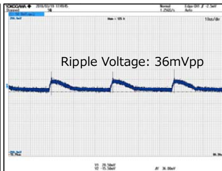
Figure 16. VOUT Ripple Voltage.2 V_{IN}=100Vac , I_{OUT}=100mA CH1: VOUT 50mV/div, 10µs/div
