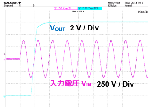
Figure 18. V_{IN} = 264 \text{ Vac} , I_{OUT} = 2 \text{ A}
