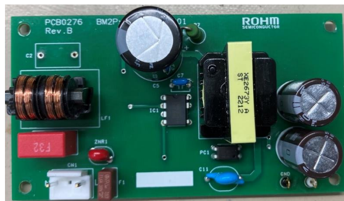
Figure 1. BM2P06B1J-EVK-001
