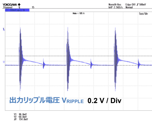
Figure 21. V_{IN} = 90 \text{ Vac} , I_{OUT} = 2 \text{ A}
