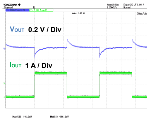
Figure 20. V_{IN} = 264 \text{ Vac} , I_{OUT} = \text{switch } 0.06 \text{ A} / 2 \text{ A}
