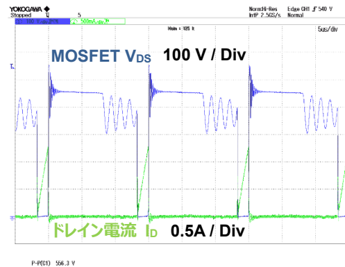
Figure 12. MOSFET波形 V_{IN} = 264 \text{ Vac} , I_{OUT} = 2 \text{ A}
