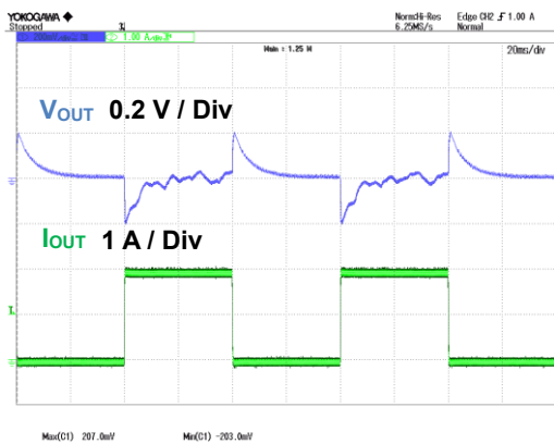
Figure 19. V_{IN} = 90 \text{ Vac} , I_{OUT} = \text{switch } 0.06 \text{ A} / 2 \text{ A}
