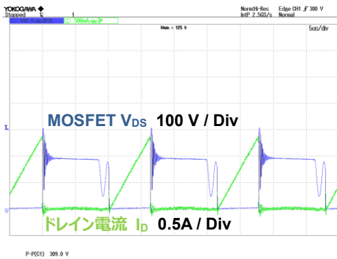
Figure 11. MOSFET波形 V_{IN} = 90 \text{ Vac} , I_{OUT} = 2 \text{ A}
