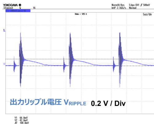
Figure 22. V_{IN} = 264 \text{ Vac} , I_{OUT} = 2 \text{ A}
