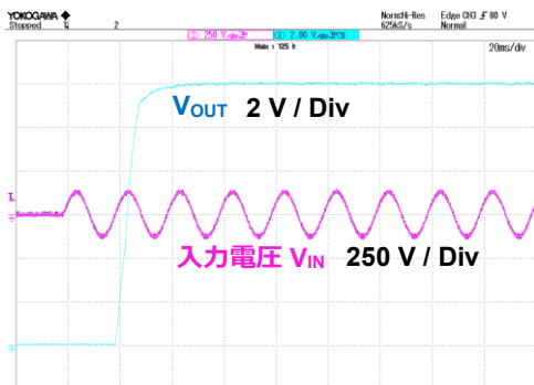
Figure 17. V_{IN} = 90 \text{ Vac} , I_{OUT} = 2 \text{ A}
