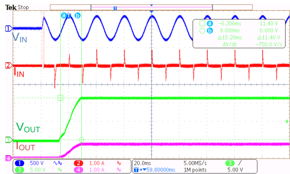
Figure 24. V_{IN} = 230 \text{ Vac} , I_{OUT} = 0.75 \text{ A}
