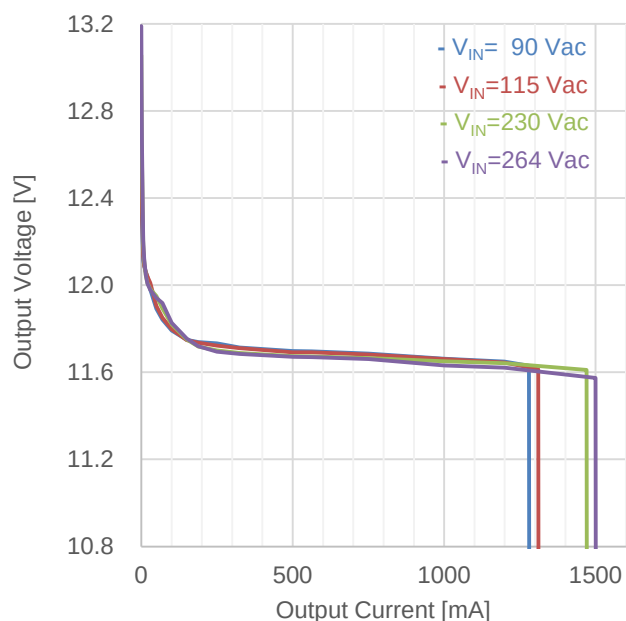
Figure 9. Load Regulation ( I_{OUT} vs V_{OUT} )
