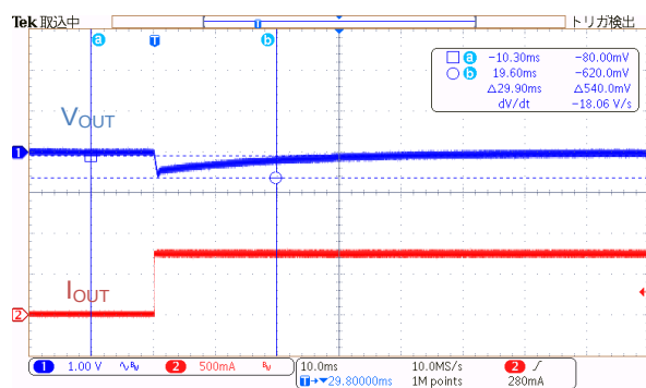
Figure 27. V_{IN} = 230 \text{ Vac} , I_{OUT} = 10 \text{ mA} \rightarrow 0.75 \text{ A}
