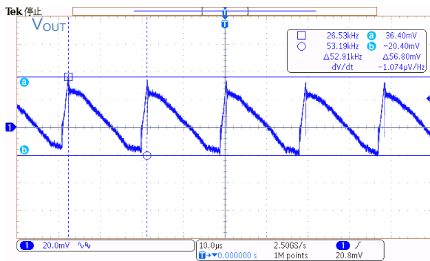
Figure 31. V_{IN} = 115 \text{ Vac} , I_{OUT} = 0.5 \text{ A}
