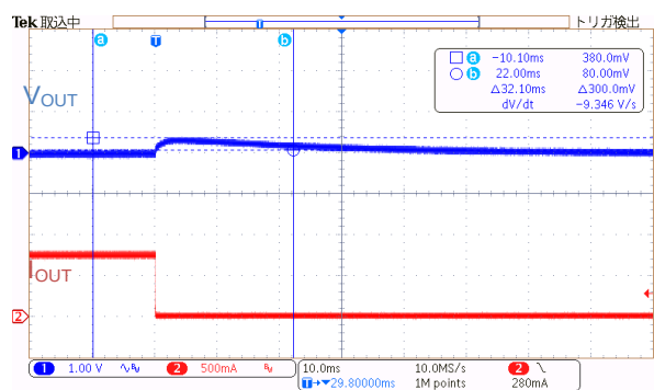
Figure 28. V_{IN} = 230 \text{ Vac} , I_{OUT} = 0.75 \text{ A} \rightarrow 10 \text{ mA}
