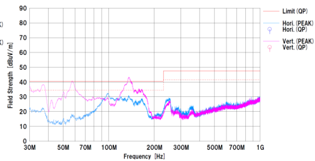
Figure 38. V IN = 230 Vac / 50 Hz, I OUT = 0.75 A QP margin = 6.2 dB
