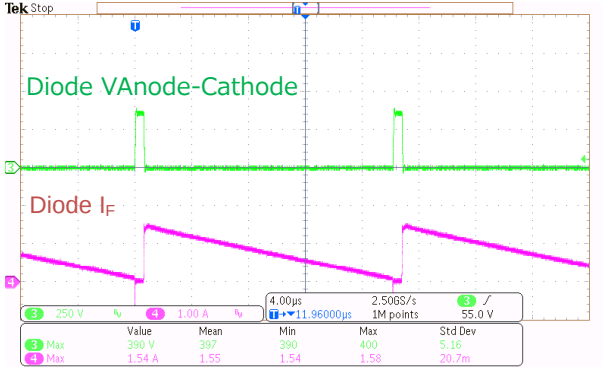
Figure 20. Diode 波形 V_{IN} = 264 \text{ Vac} , I_{OUT} = 0.75 \text{ A}
