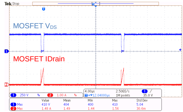
Figure 19. MOSFET 波形 V_{IN} = 264 \text{ Vac} , I_{OUT} = 0.75 \text{ A}
