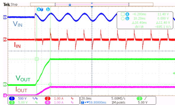
Figure 23. V_{IN} = 115 \text{ Vac} , I_{OUT} = 0.75 \text{ A}
