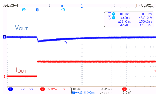
Figure 25. V_{IN} = 115 \text{ Vac} , I_{OUT} = 10 \text{ mA} \rightarrow 0.75 \text{ A}
