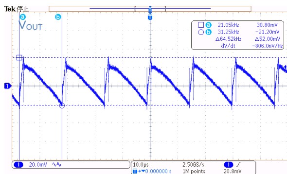
Figure 33. V_{IN} = 115 \text{ Vac} , I_{OUT} = 0.75 \text{ A}
