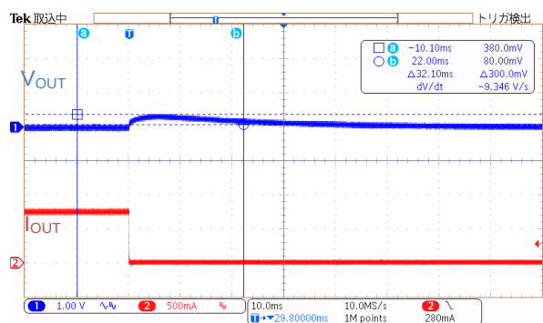
Figure 26. V_{IN} = 115 \text{ Vac} , I_{OUT} = 0.75 \text{ A} \rightarrow 10 \text{ mA}
