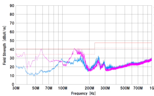
Figure 37. V IN = 110 Vac / 60 Hz, I OUT = 0.75 A QP margin = 7.3 dB
