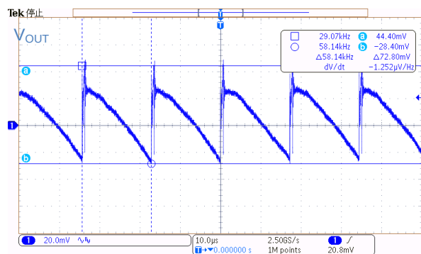
Figure 34. V_{IN} = 230 \text{ Vac} , I_{OUT} = 0.75 \text{ A}
