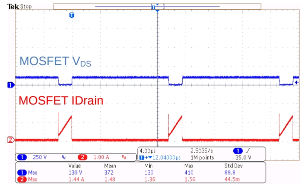
Figure 17. MOSFET 波形 V_{IN} = 90 \text{ Vac} , I_{OUT} = 0.75 \text{ A}
