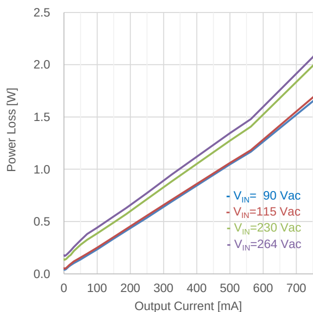
Figure 11. Load Regulation ( I_{OUT} vs P_{LOSS} )
