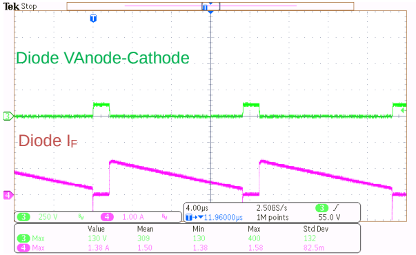
Figure 18. Diode 波形 V_{IN} = 90 \text{ Vac} , I_{OUT} = 0.75 \text{ A}
