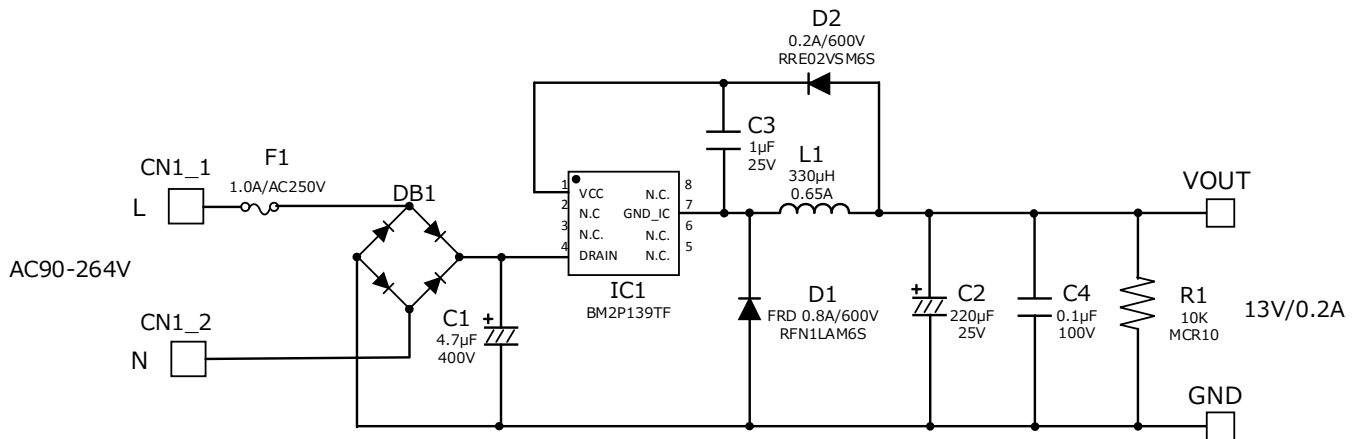
Figure 23. BM2P139TF-EVK-001 回路図
