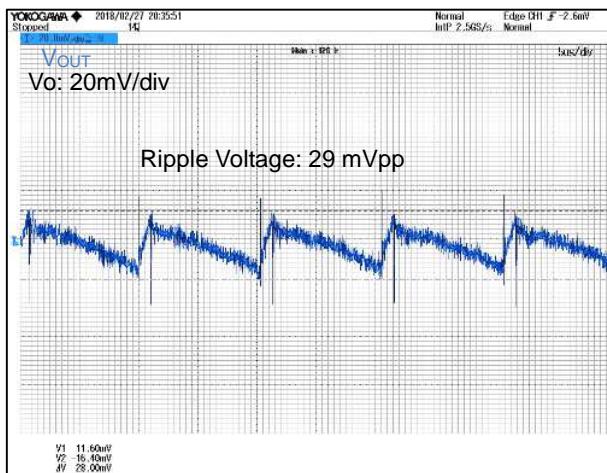
Figure 19. V_{IN} = 115 \text{ Vac} , I_{OUT} = 0.15 \text{ A}
