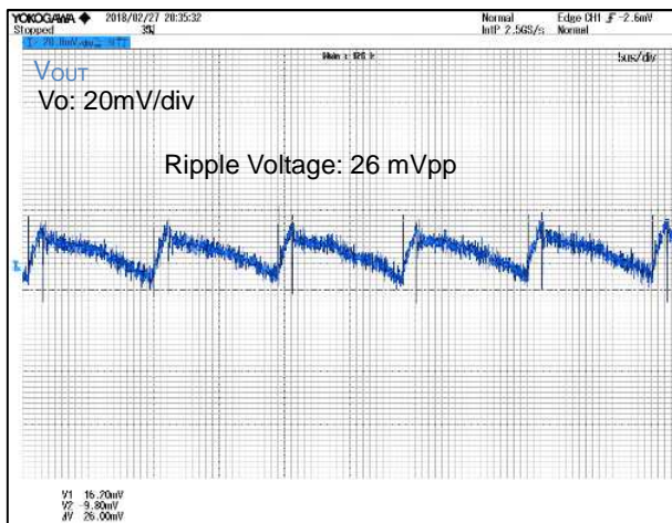
Figure 21. V_{IN} = 115 \text{ Vac} , I_{OUT} = 0.20 \text{ A}
