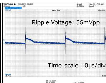
V_{IN}=230Vac, I_{OUT}=100mA
