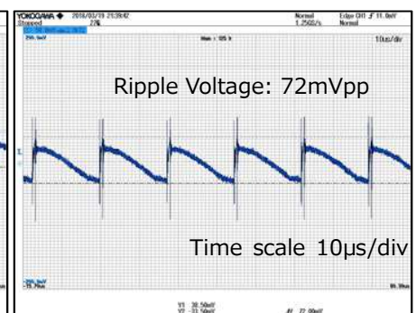
V_{IN}=230Vac, I_{OUT}=600mA
