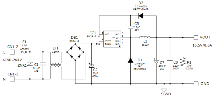
Figure 3. BM2P161W-EVK-001 回路図
