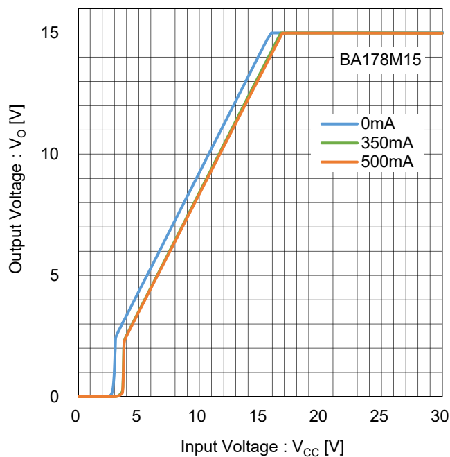
Figure 85. 出力電圧 vs 入力電圧 Test Circuit A
