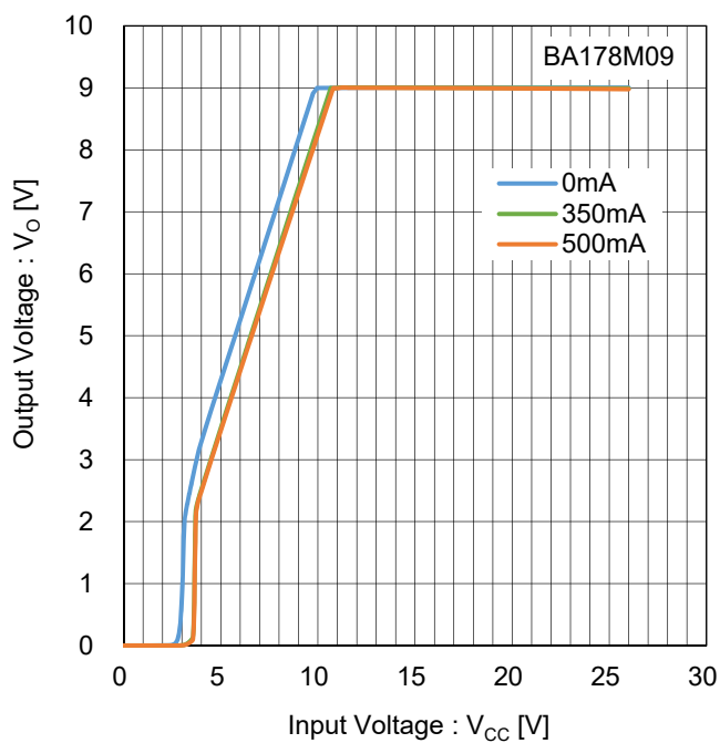
Figure 49. 出力電圧 vs 入力電圧 Test Circuit A
