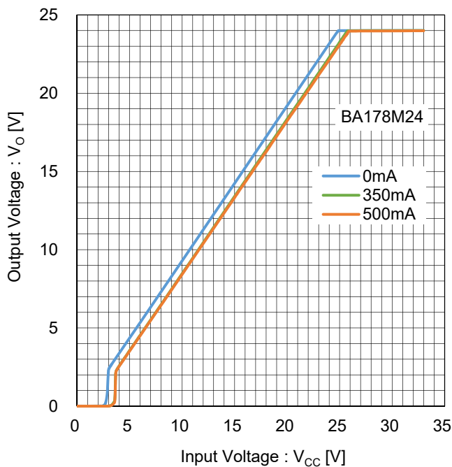
Figure 121. 出力電圧 vs 入力電圧 Test Circuit A
