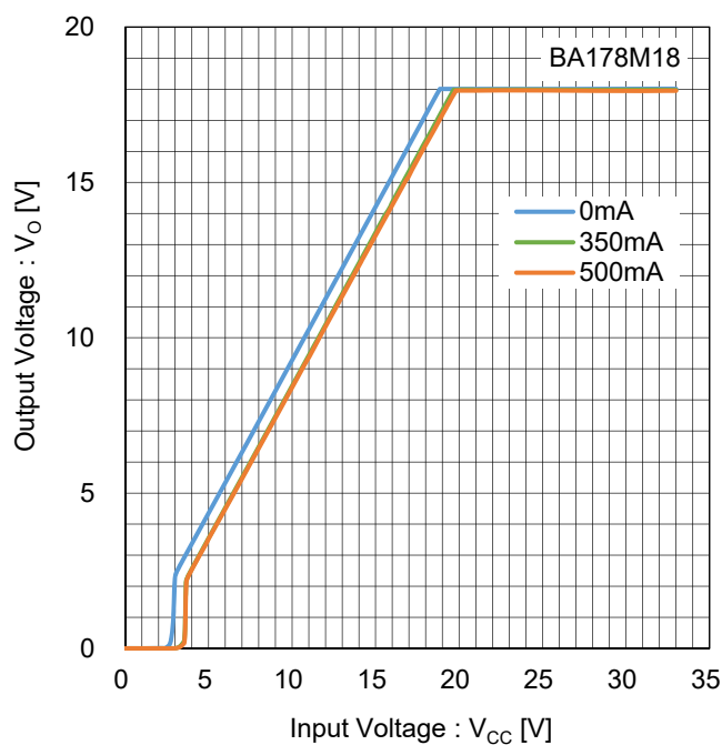
Figure 97. 出力電圧 vs 入力電圧 Test Circuit A
