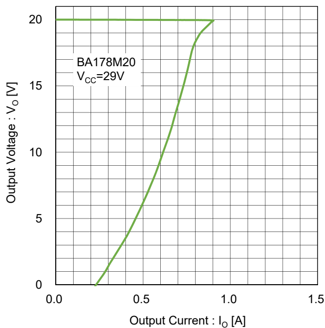
Figure 111. 過電流保護 Test Circuit C
