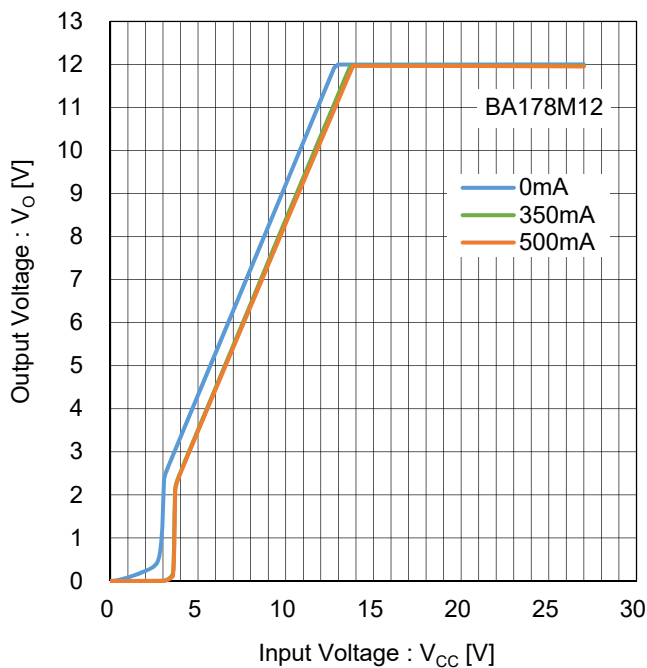
Figure 73. 出力電圧 vs 入力電圧 Test Circuit A
