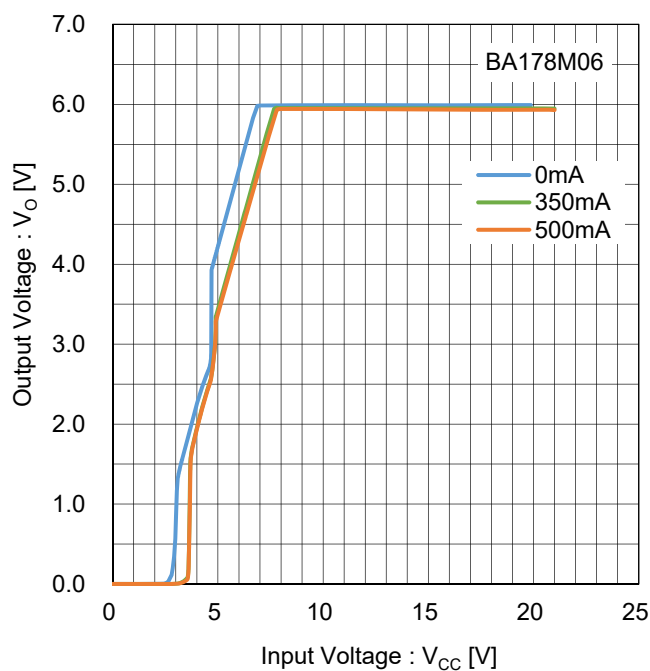
Figure 13. 出力電圧 vs 入力電圧 Test Circuit A
