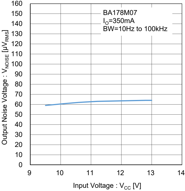
Figure 36. 出カノイズ電圧 Test Circuit L
