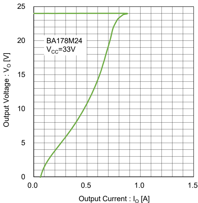
Figure 123. 過電流保護 Test Circuit C
