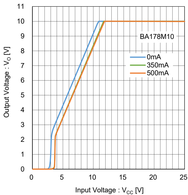
Figure 61. 出力電圧 vs 入力電圧 Test Circuit A
