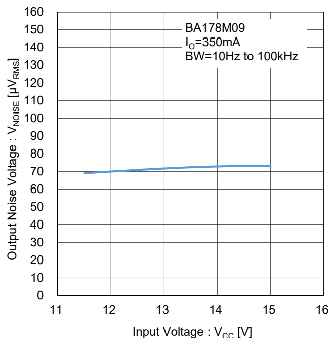
Figure 60. 出カノイズ電圧 Test Circuit L
