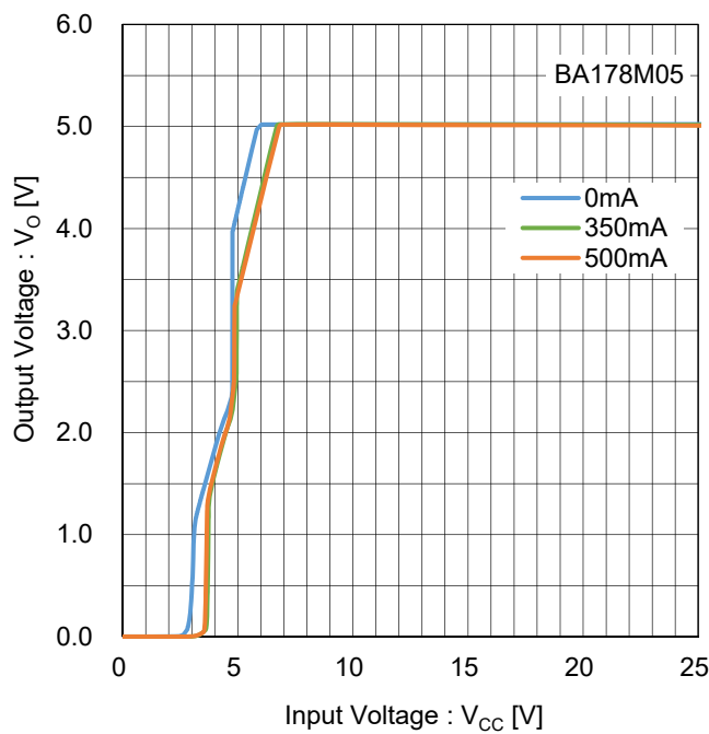
Figure 1. 出力電圧 vs 入力電圧 Test Circuit A
