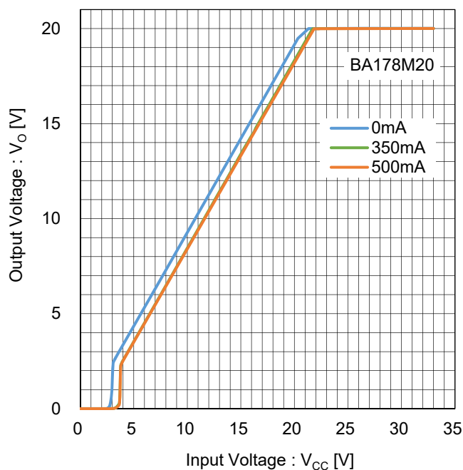
Figure 109. 出力電圧 vs 入力電圧 Test Circuit A
