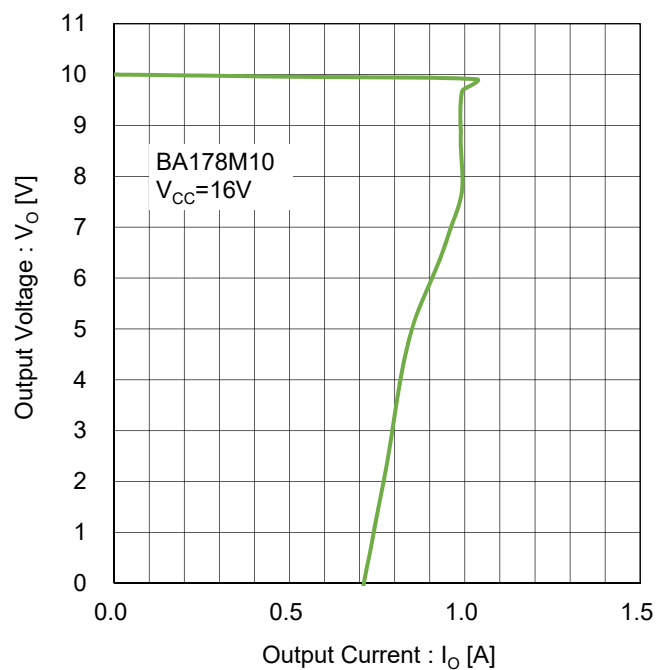
Figure 63. 過電流保護 Test Circuit C
