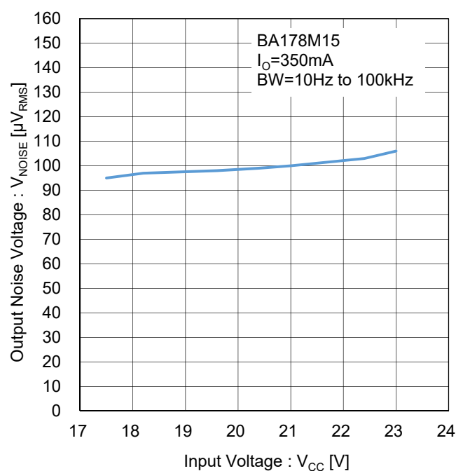
Figure 96. 出カノイズ電圧 Test Circuit L
