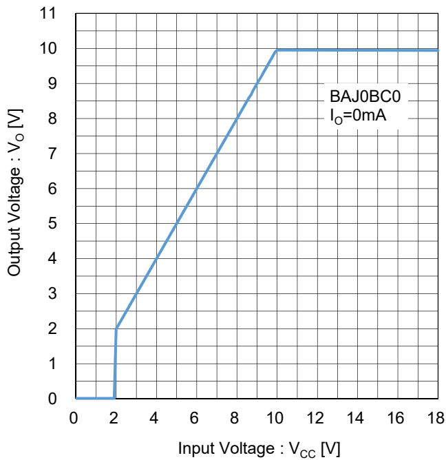
Figure 153. 出力電圧 vs 入力電圧 ( I_o=0mA ) Test Circuit C
