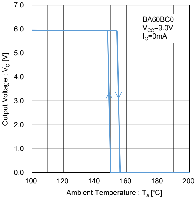
Figure 105. 過熱保護 Test Circuit M
