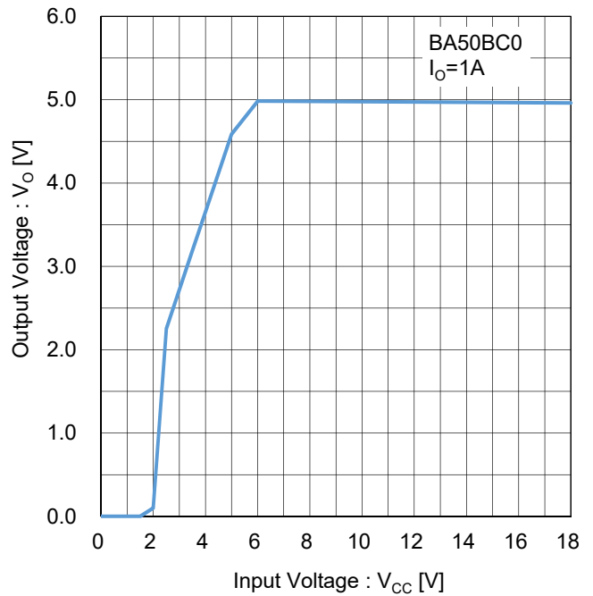
Figure 79. 出力電圧 vs 入力電圧 ( I_o=1A ) Test Circuit C
