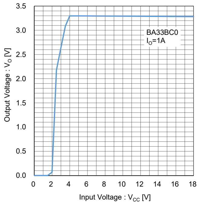
Figure 64. 出力電圧 vs 入力電圧 ( I_o=1A ) Test Circuit C
