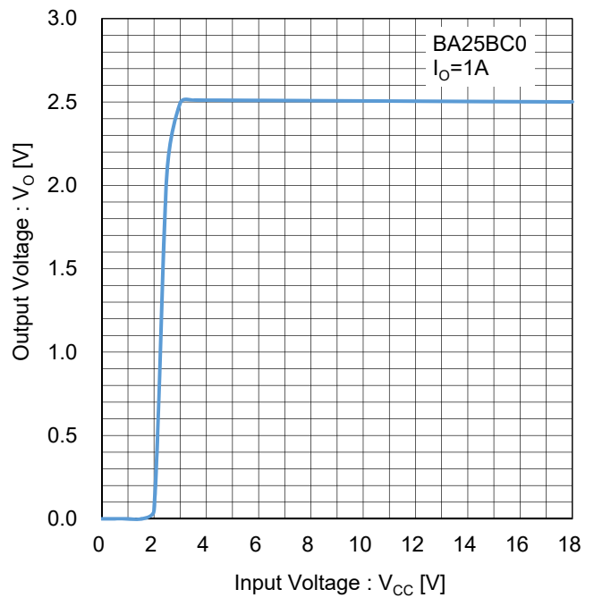
Figure 34. 出力電圧 vs 入力電圧 ( I_o=1A ) Test Circuit C
