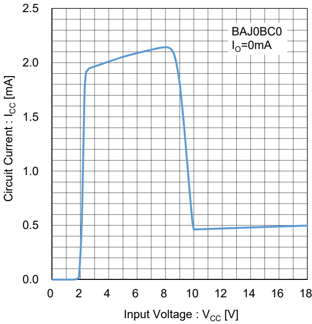
Figure 151. 回路電流 Test Circuit A
