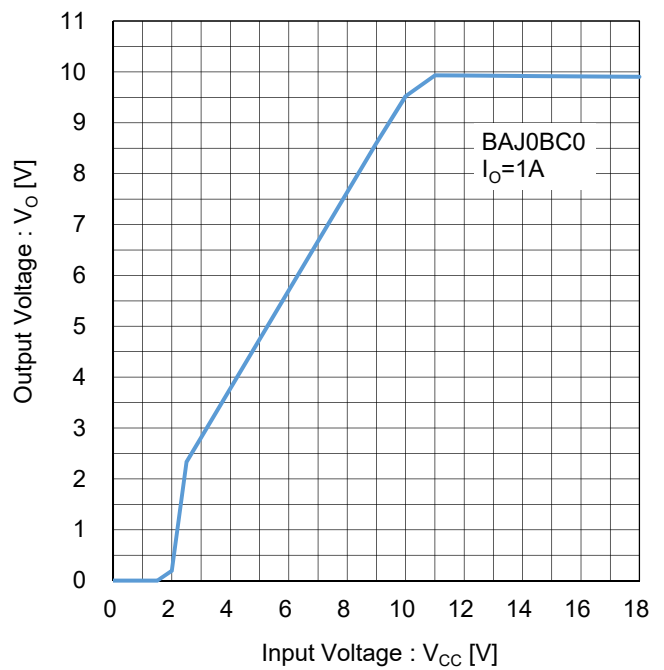
Figure 154. 出力電圧 vs 入力電圧 ( I_o=1A ) Test Circuit C
