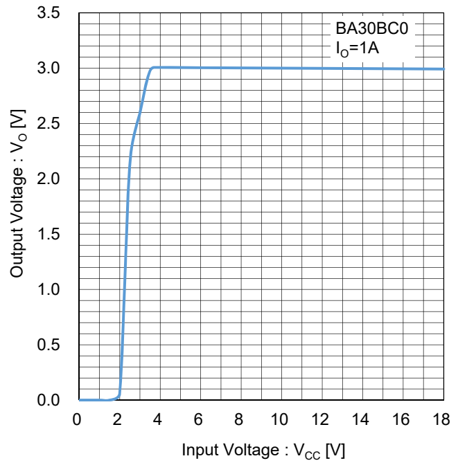
Figure 49. 出力電圧 vs 入力電圧 ( I_o=1A ) Test Circuit C
