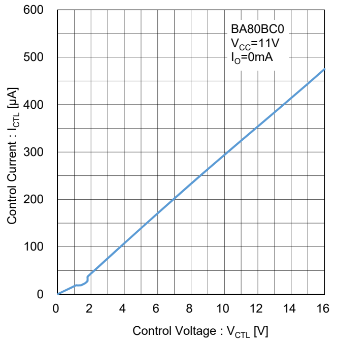
Figure 134. CTL ピン流入電流 Test Circuit L
