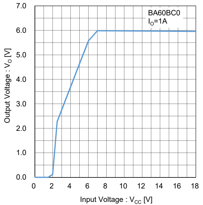
Figure 94. 出力電圧 vs 入力電圧 ( I_o=1A ) Test Circuit C
