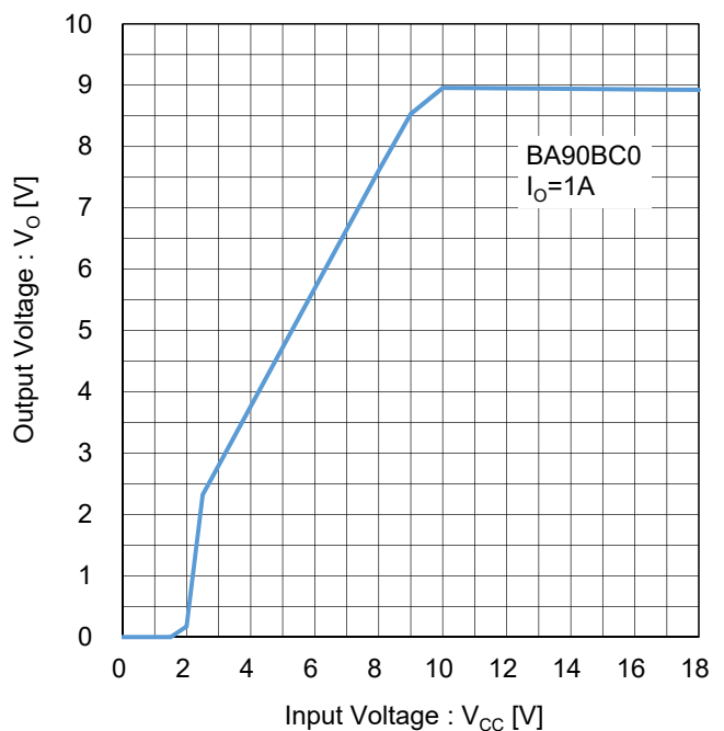
Figure 139. 出力電圧 vs 入力電圧 ( I_o=1A ) Test Circuit C
