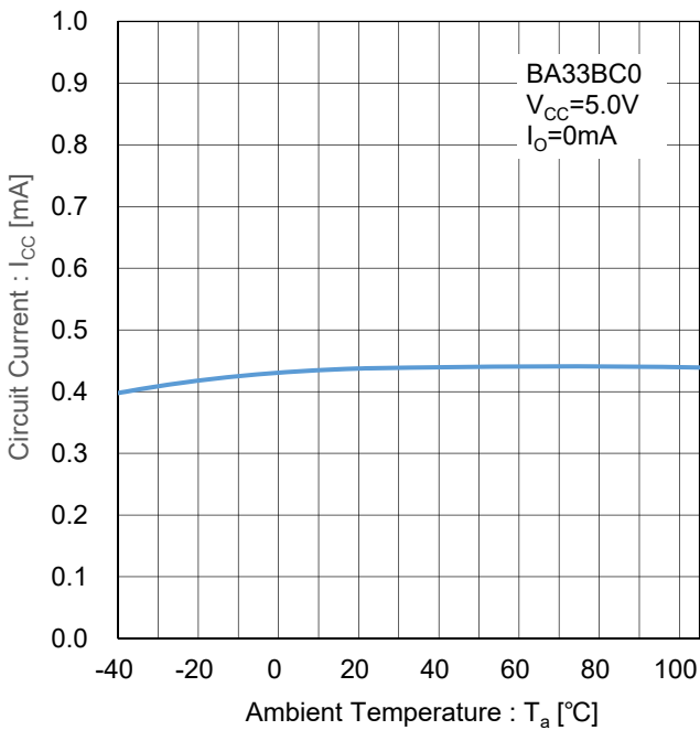
Figure 71. 回路電流 vs 温度 Test Circuit I
