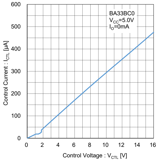
Figure 74. CTL ピン流入電流 Test Circuit L
