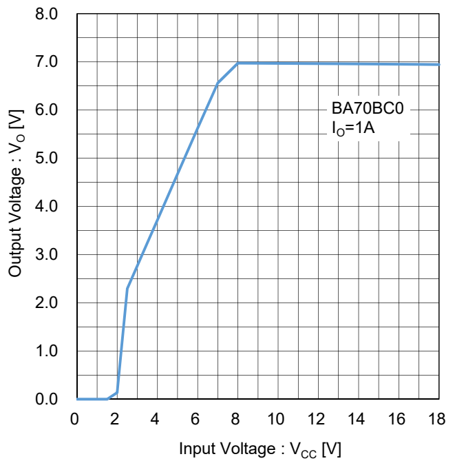
Figure 109. 出力電圧 vs 入力電圧 ( I_o=1A ) Test Circuit C
