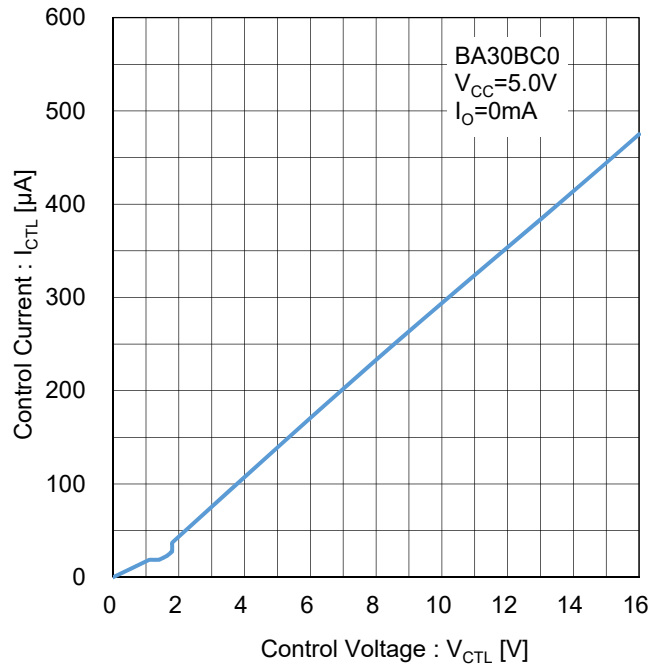
Figure 59. CTL ピン流入電流 Test Circuit L
