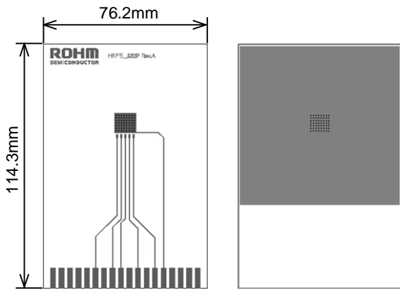
Figure 11-8. Top Layer Trace
