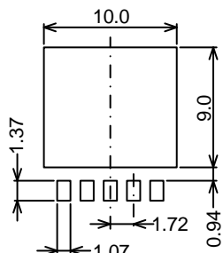
Figure 11-2. Footprint
