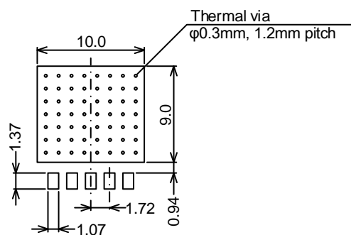
Figure 11-6. Footprint
