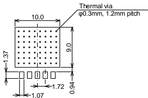
Figure 11-12. Footprint
