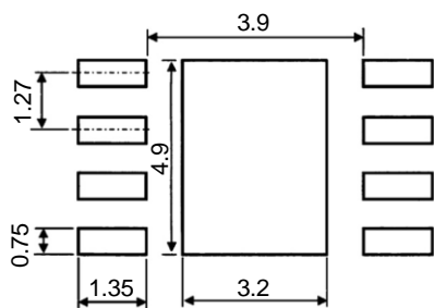
Figure 11-2. Footprint
