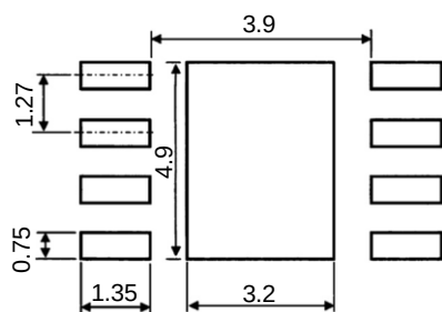
Figure 11-2. Footprint
