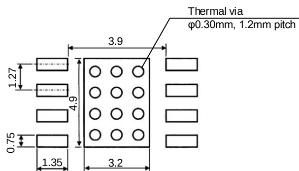
Figure 11-6. Footprint
