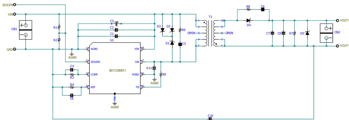
Figure 4. BD7J200EFJ-EVK-002 回路図
