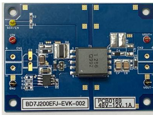
Figure 1. BD7J200EFJ-EVK-002 Top View
