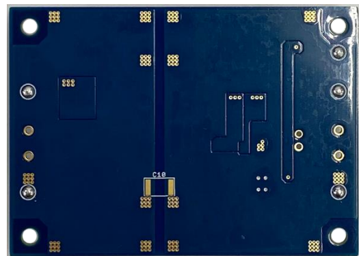
Figure 2. BD7J200EFJ-EVK-002 Bottom View
