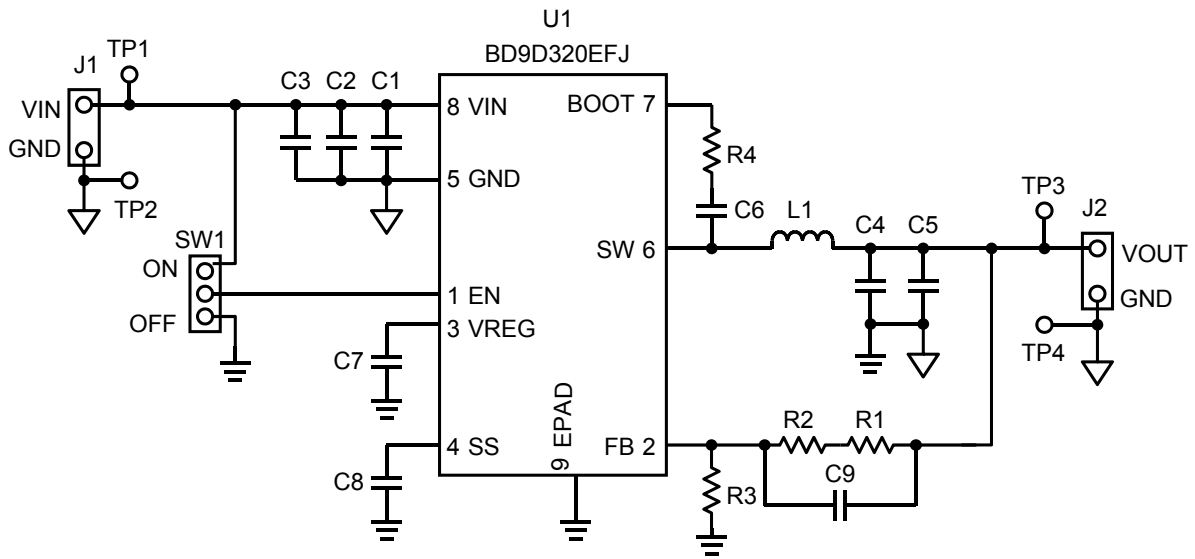
Figure 2. BD9D320EFJ-EVK-001 回路図
