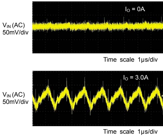
Figure 13. 入力電圧リップル波形 V_{IN} = 12V, V_O = 3.3V
