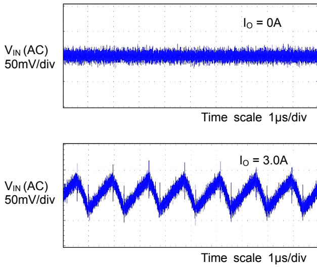
Figure 13. 入力電圧リップル波形 V_{IN} = 12V, V_O = 3.3V
