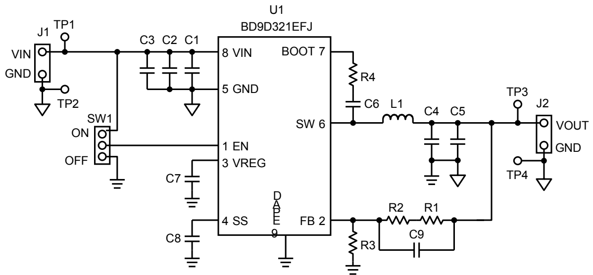
Figure 2. BD9D321EFJ-EVK-001 回路図
