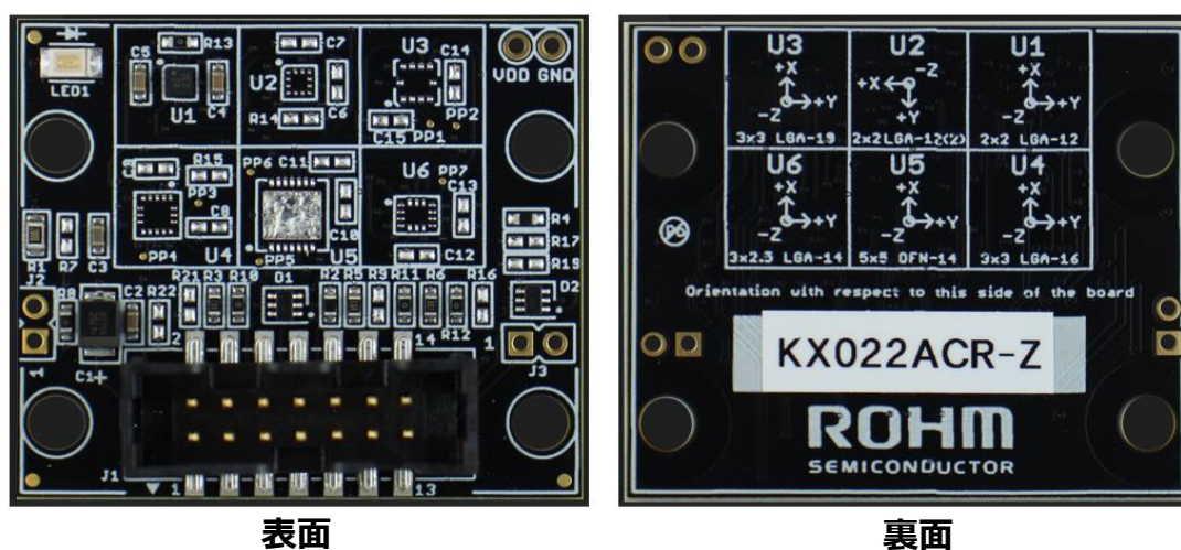
Figure 1: KX022ACR-EVK-001 写真
