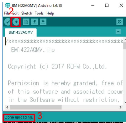
Figure 4. Upload 画面
