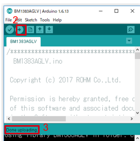
Figure 4. Upload 画面
