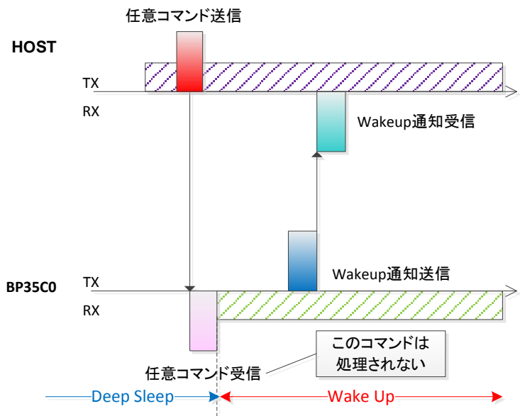
図 10 DeepSleep → Wakeup
