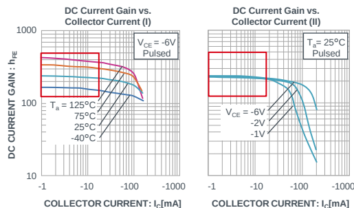
2SA1576U3 (PNP)
