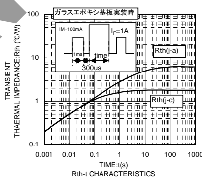
R_{th}-t CHARACTERISTICS
