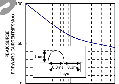
IFSM-CYCLE CHARACTERISTICS
