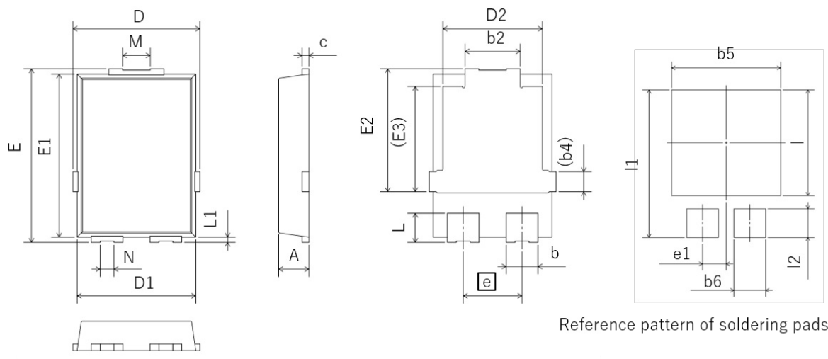
TO-277A, (TO-277GE)
