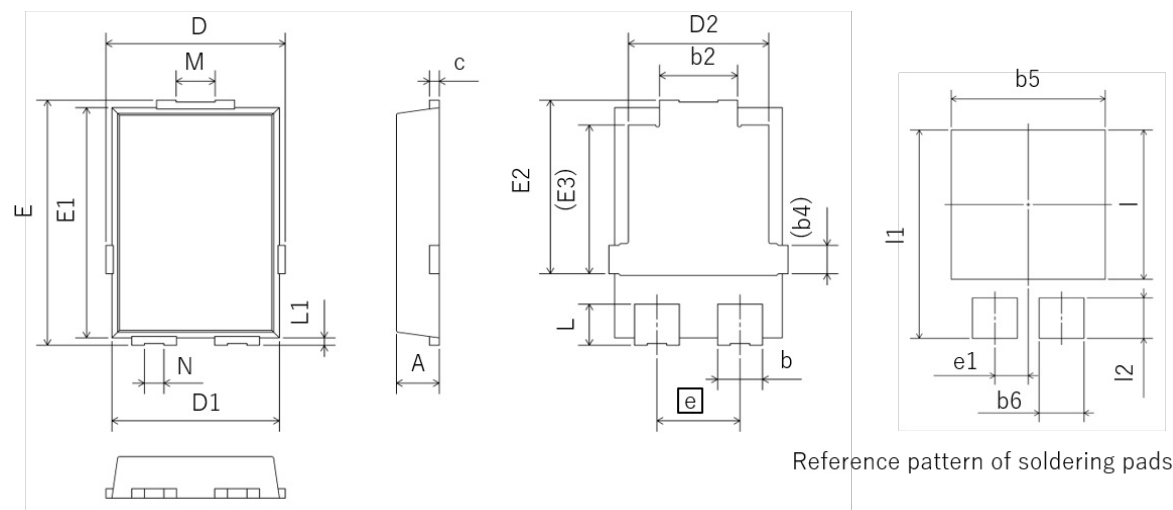
TO-277A, (TO-277GE)
